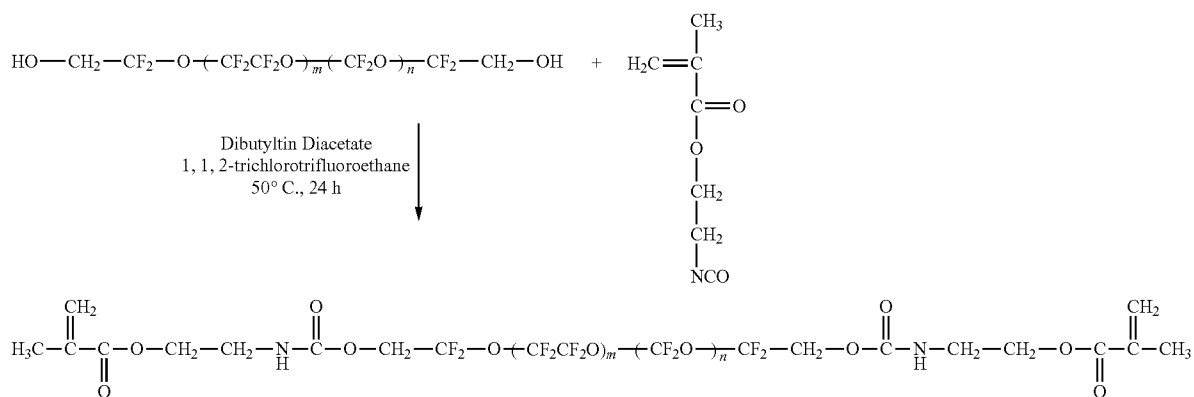
Scheme 1. Synthesis and Photocuring of Functionalized Perfluoropolyethers.
