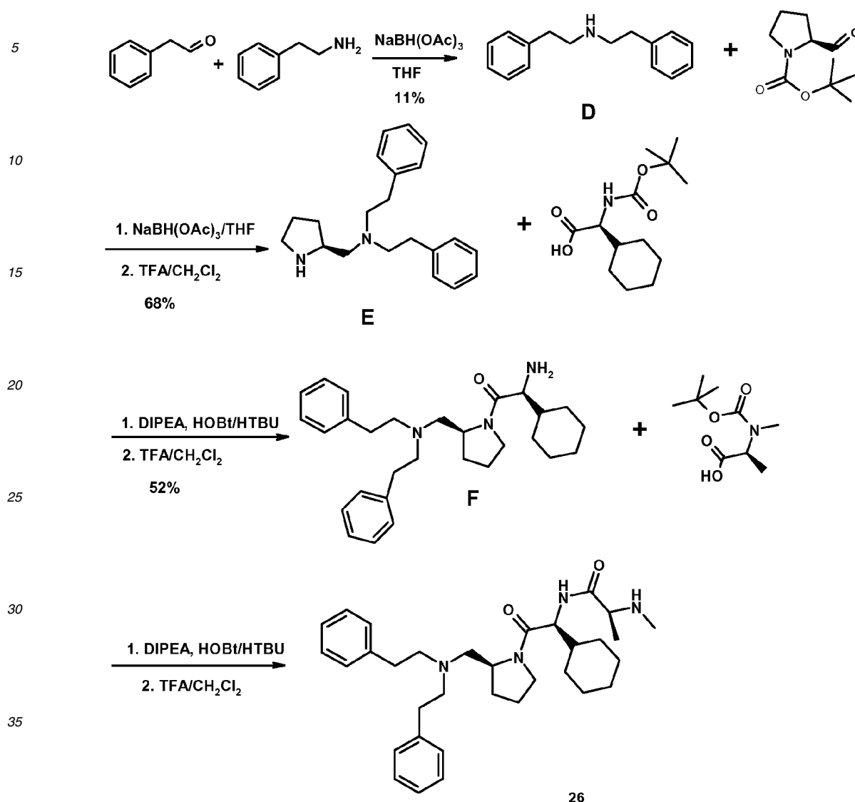
Scheme 6
