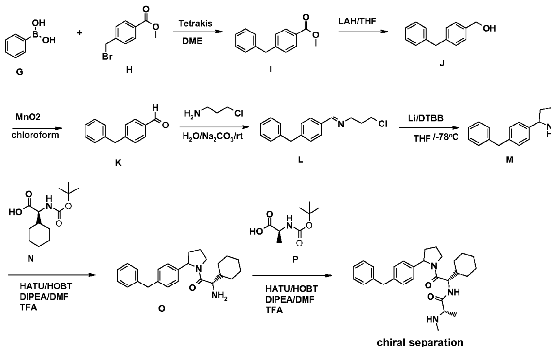
Scheme 7
