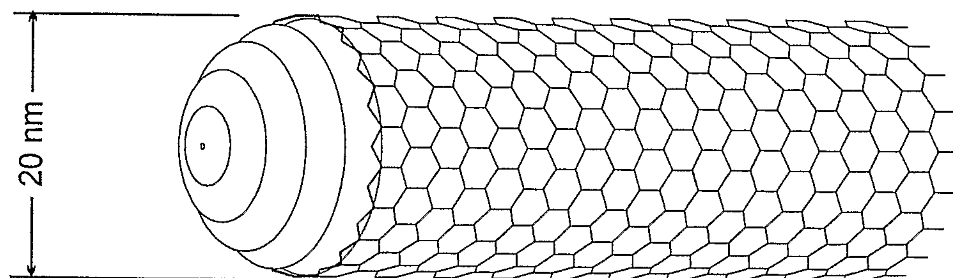
FIG. 2 (A) CLOSED-END MWCNT
