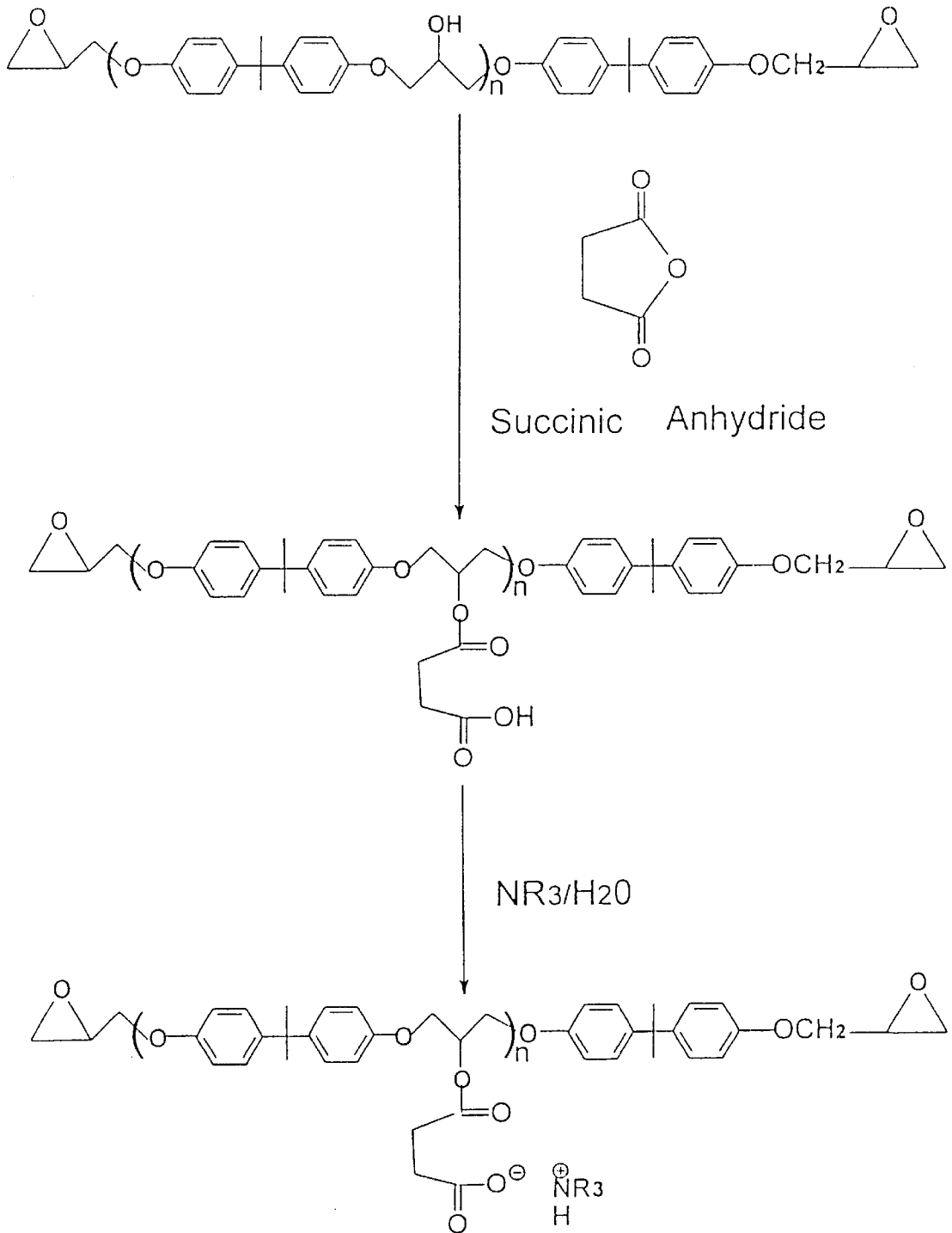
Figure 1. Preparation of self-emulsified aqueous epoxy resin
