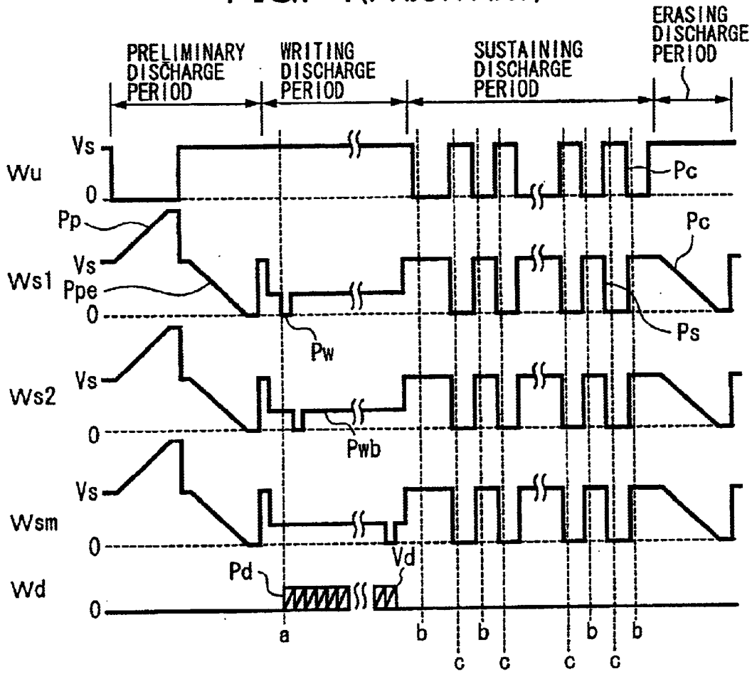
FIG. 4(PRIOR ART)
