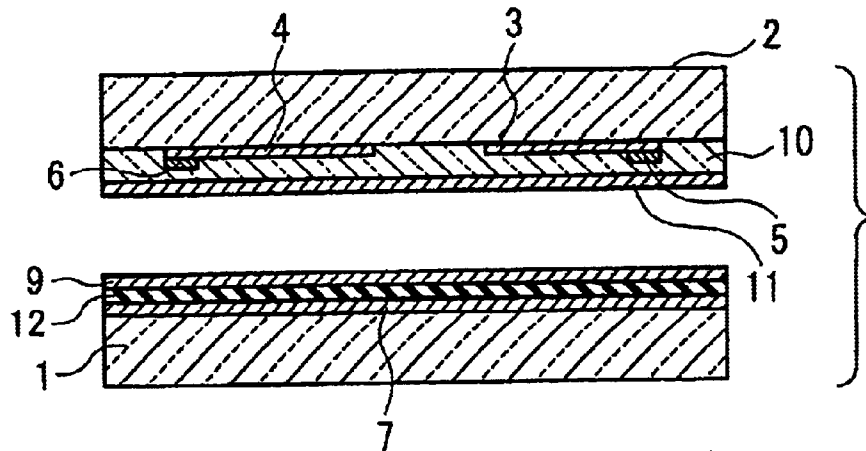
FIG. 5(PRIOR ART)
