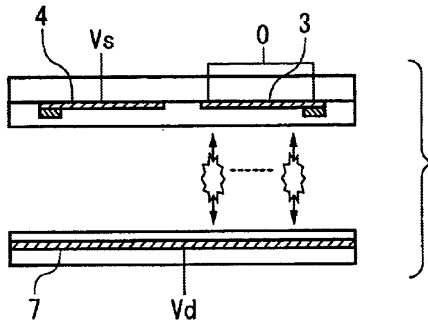
FIG. 6(PRIOR ART)
