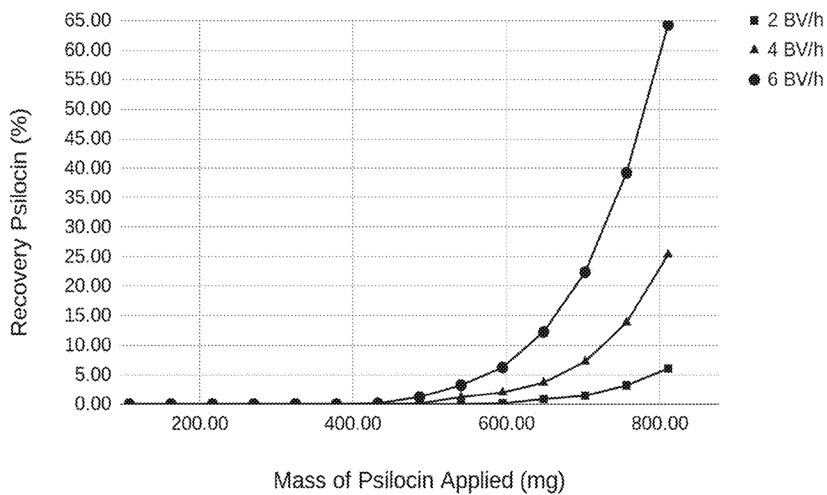
XAD4 Adsorption Breakthrough Experiments
