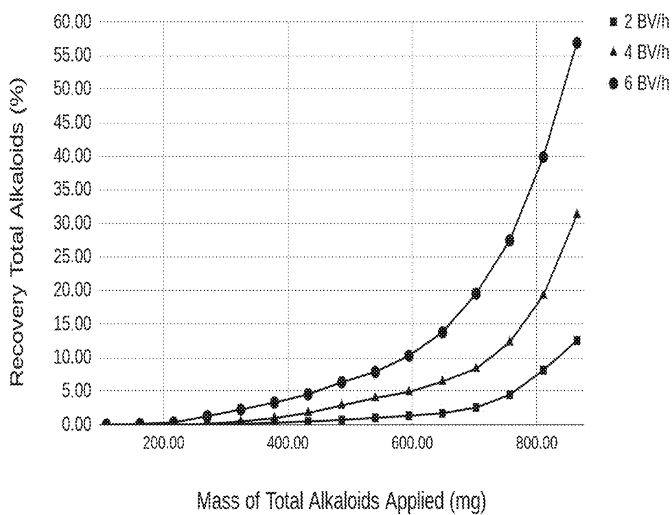
XAD4 Adsorption Breakthrough Experiments
