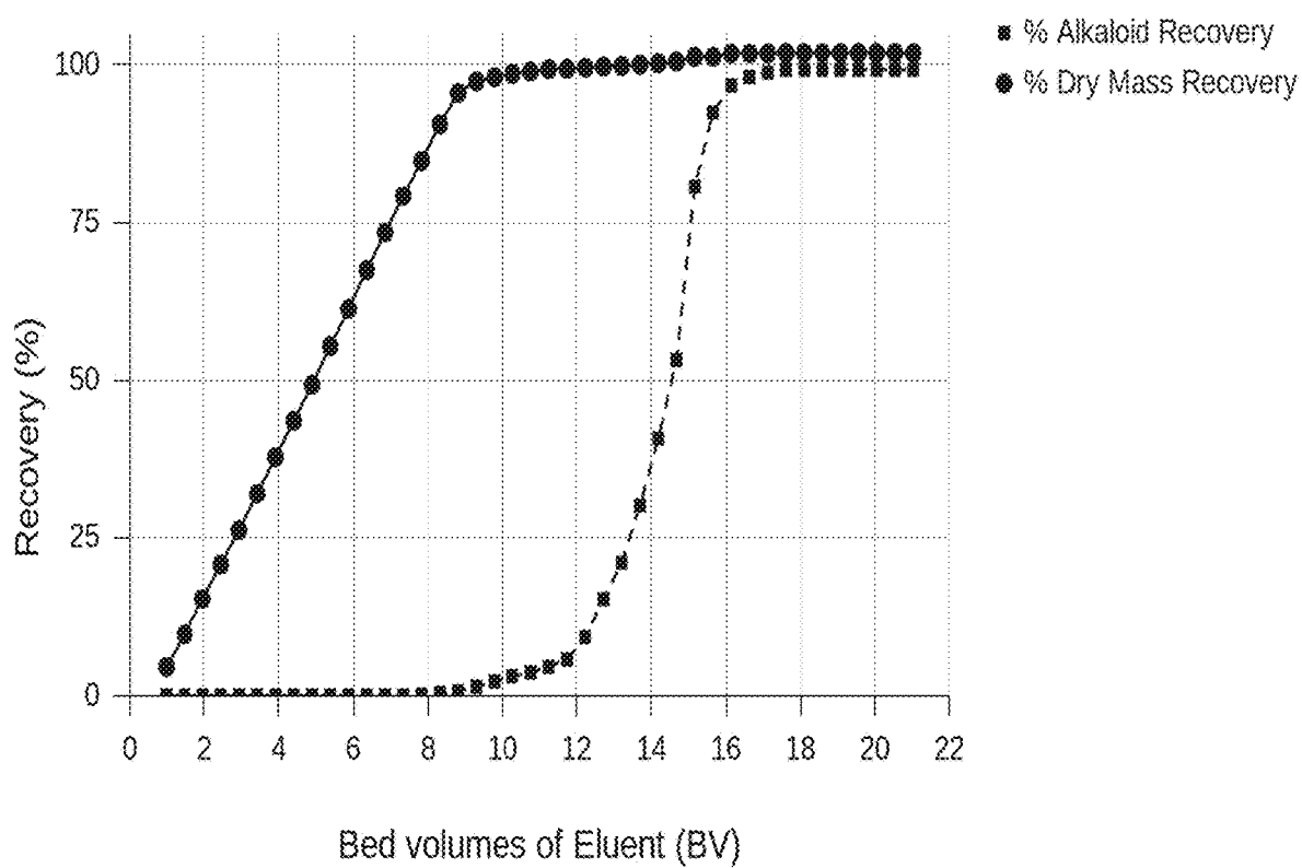
Recovery of Psilocybin on XAD4
