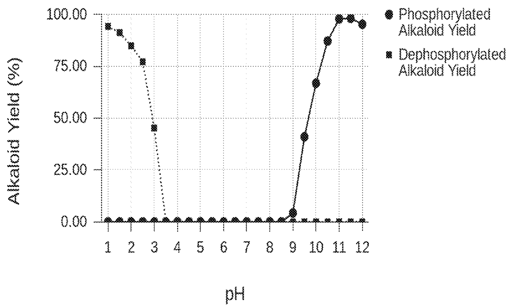
Effect of pH on Alkaloid Extraction Yield
