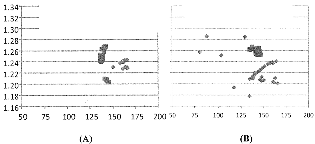
Figure 8. Relationship between refractive index and thickness of anti-reflection thin film (A: anti reflection solar float glass; B: anti reflection matte glass).
