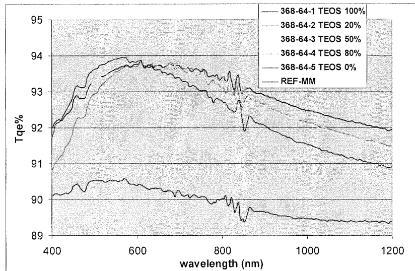
Figure 9. Transmittance spectra of anti-reflection matte glass from blended sols (Tqe% of raw matte glass is included as the bottom plot for reference and the labels are those in Table 5).
