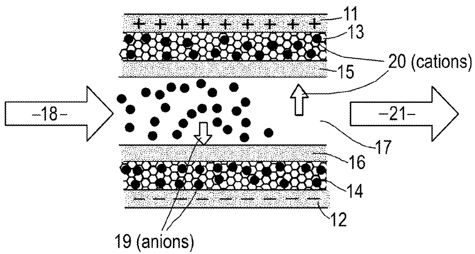
CDI Assembly
