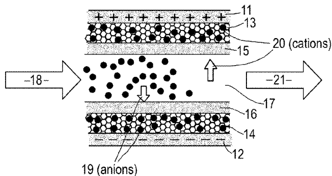
CDI Assembly
