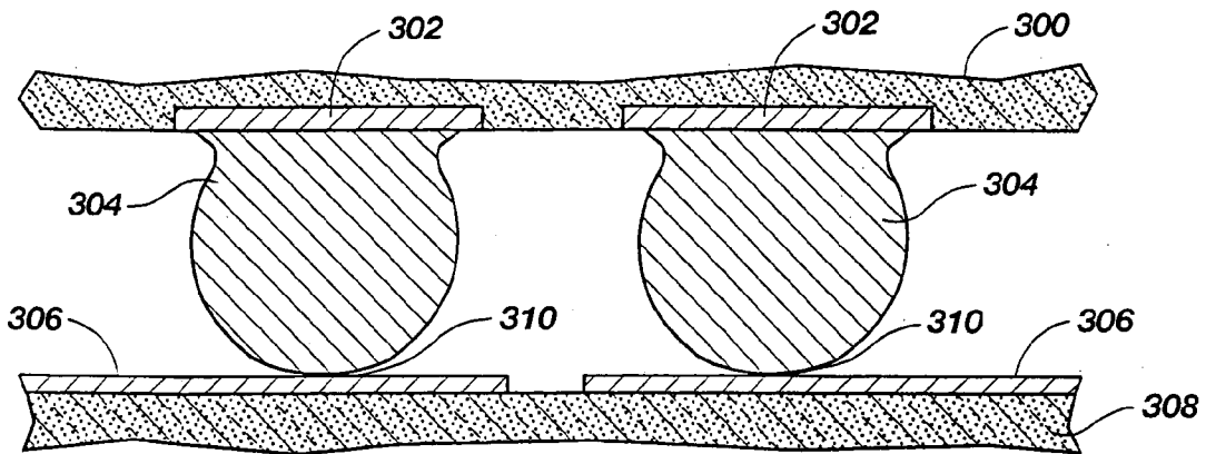
Fig. 31 (PRIOR ART)
