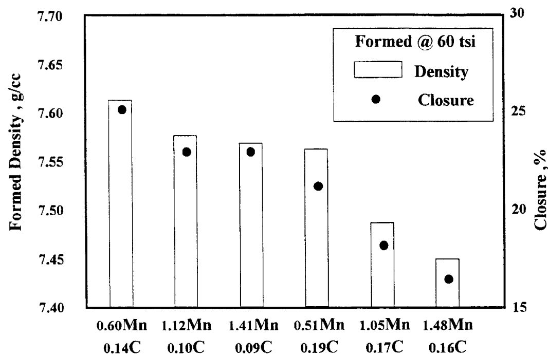
Figure 7 : High Density Forming Of FeCMn Rings
