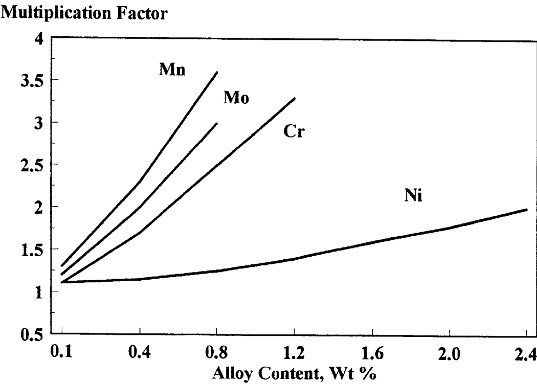
Figure 9 : The effect of alloying elements on the hardenability of steel.
