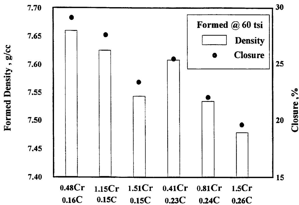
Figure 5 : High Density Forming Of FeCCr Rings
