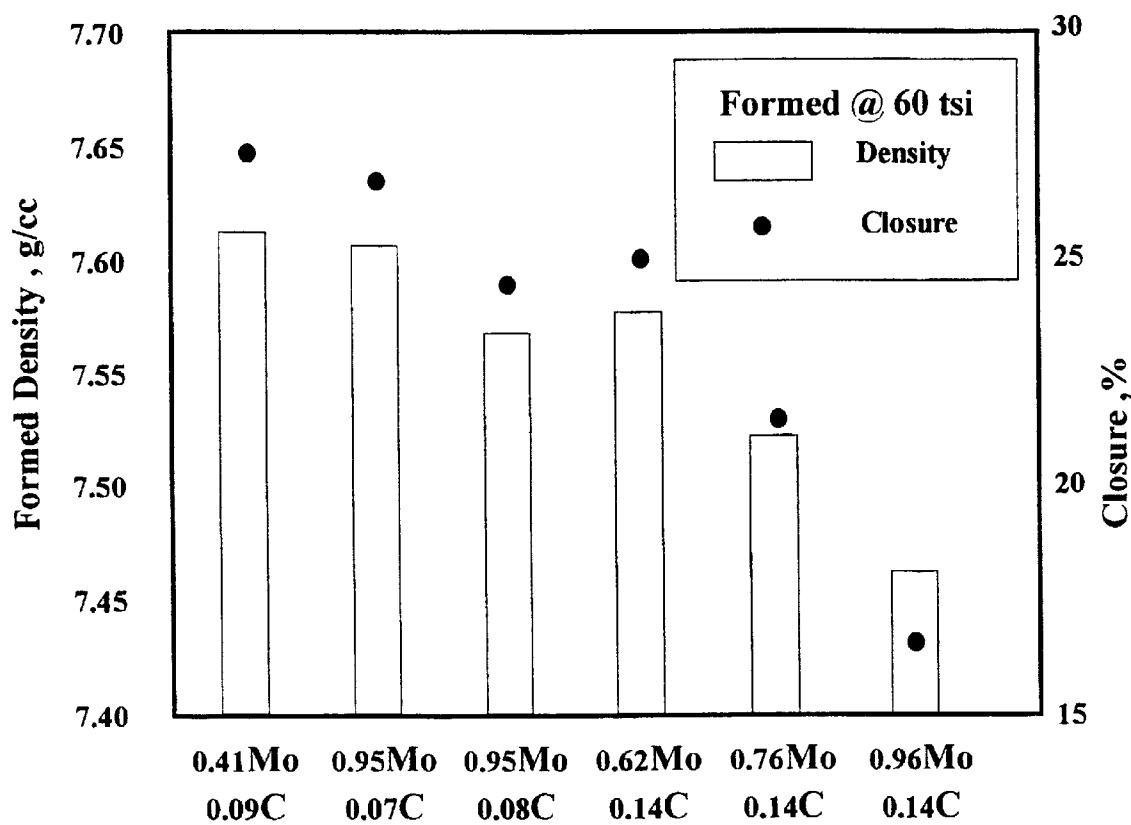
Figure 6 : High Density Forming Of FeCMo Rings
