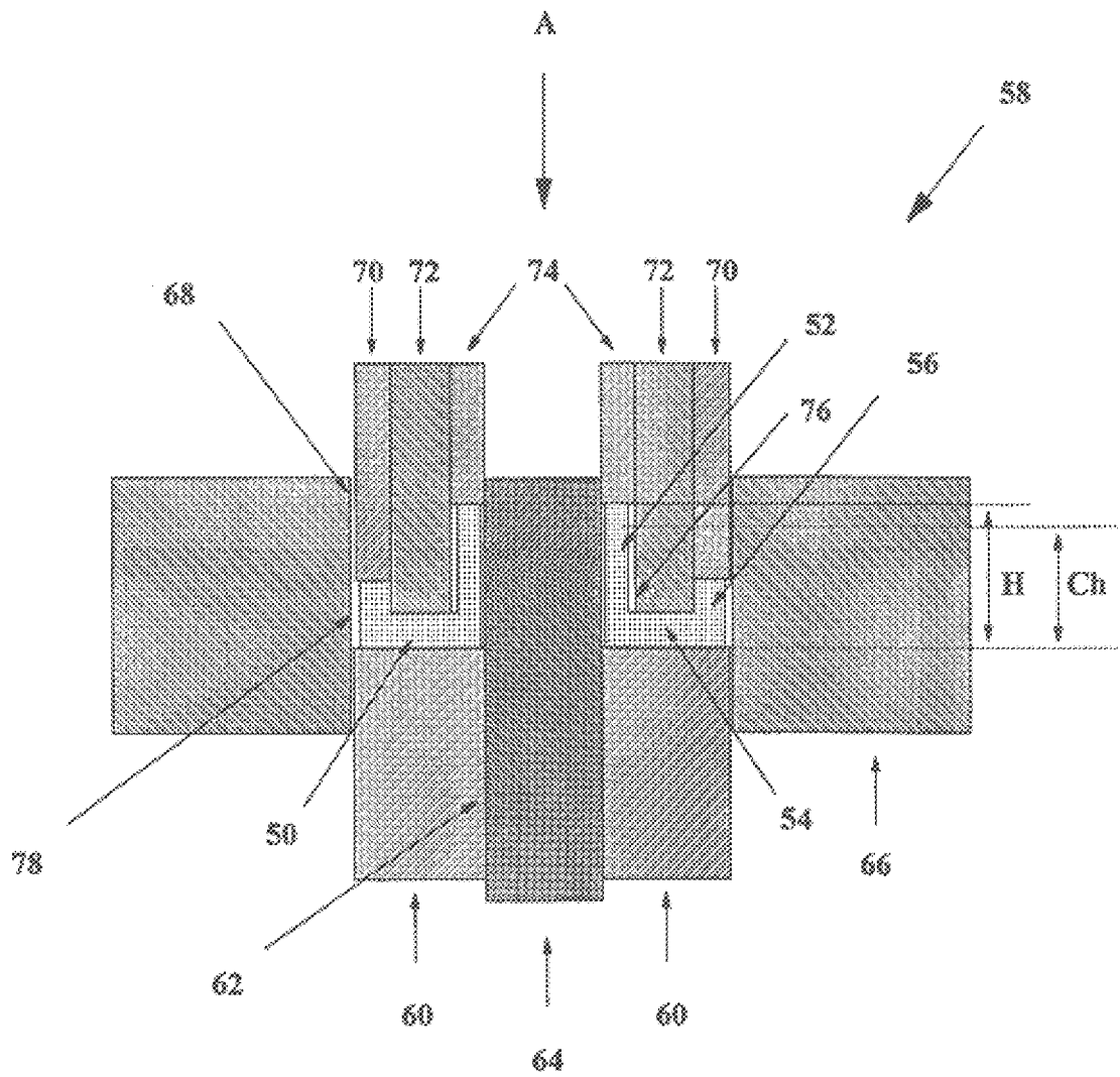
Figure 14 : Cross sectional view of the forming process for a multilevel component
