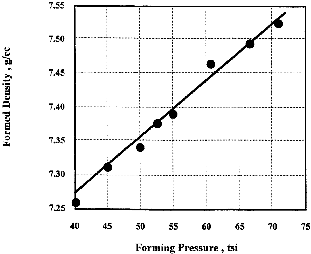
Figure 3 : High Density Forming Of FeCMn Test Bars
