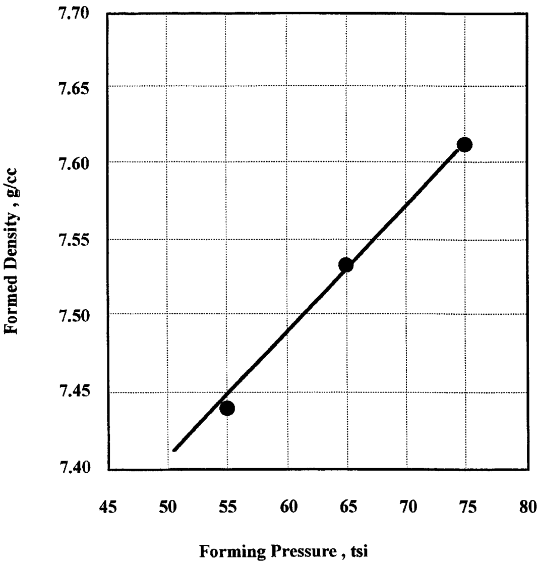
Figure 13 : High Density Forming Of FeCMo Rings (QMP 4401 0.85%Mo Prealloy + 0.2%C)
