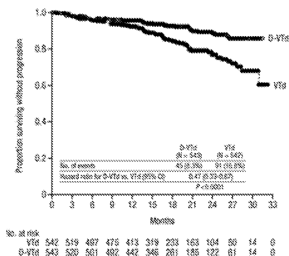
Figure 2: Kaplan-Meier Curve of PFS in CASSIOPEIA 17
