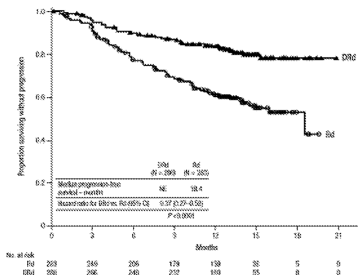
Figure 3: Kaplan-Meier Curve of PFS in POLLUX
