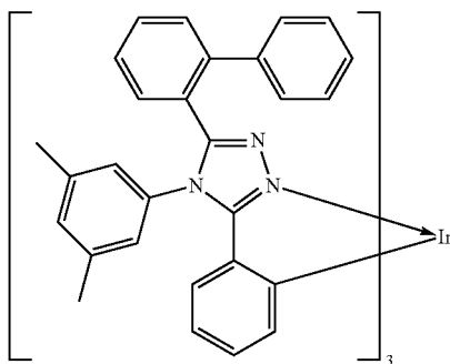
Step 3: Synthesis of tris{2-[5-(biphenyl-2-yl)-4-(3,5-dimethylphenyl)-4H-1,2,4-triazol-3-yl-kappaN 2 ]phenyl-kappaC 1 }iridium
