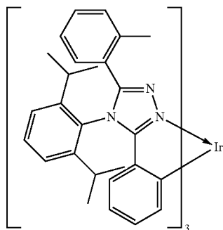
Step 5: Synthesis of tris(2-{4-[2,6-di(propan-2-yl)phenyl]-5-(2-methylphenyl)-4H-1,2,4-triazol-3-yl-kN 2 }phenyl-kC 1 )iridium
