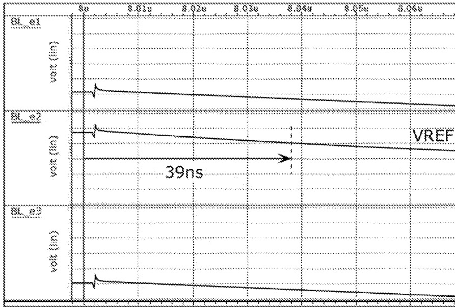
When accessing BL_e2
