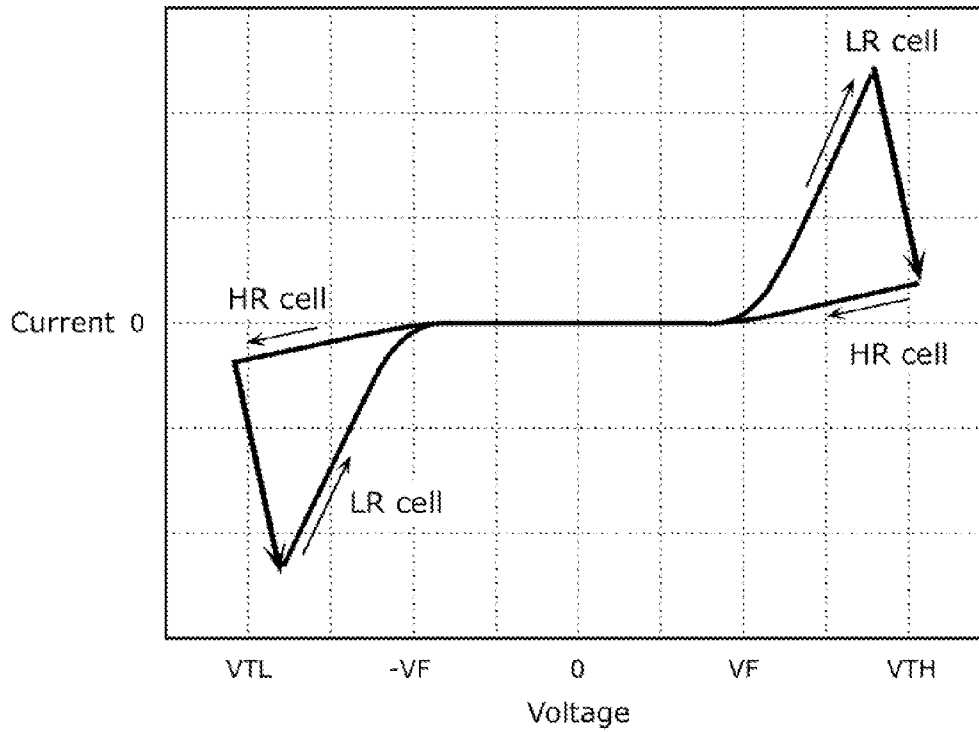
Memory cell current characteristic
