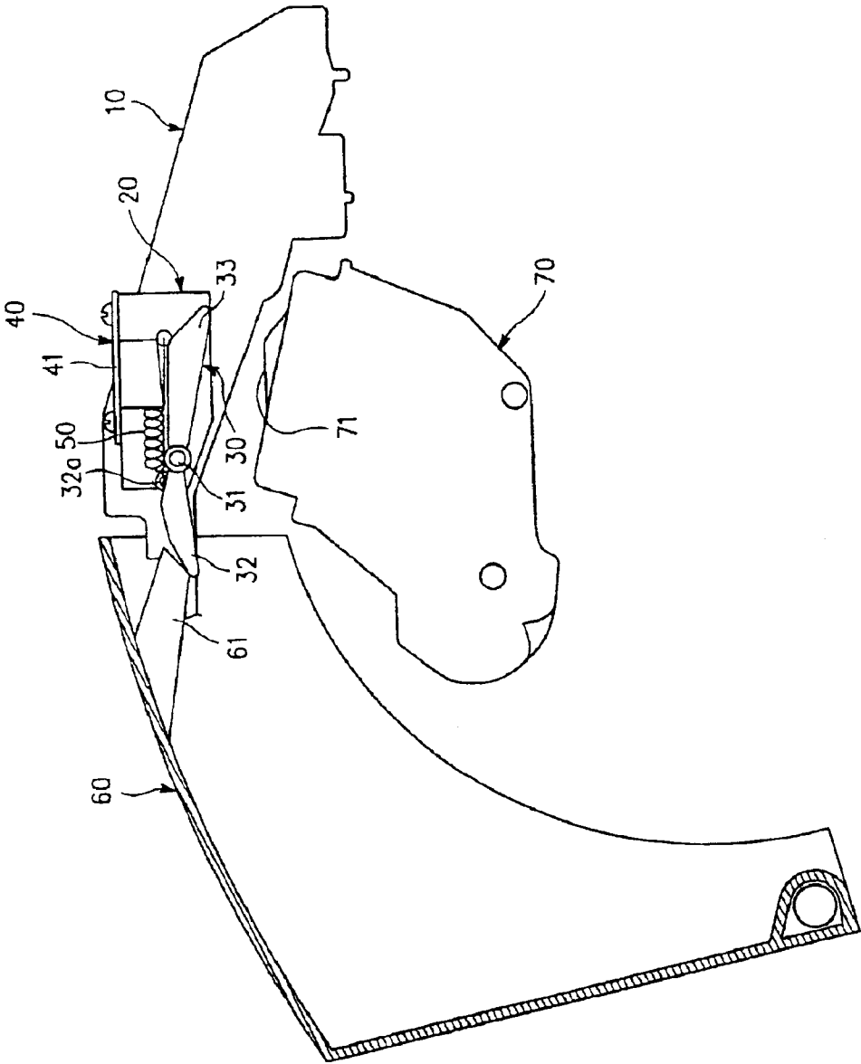
FIG. 4 (PRIOR ART)
