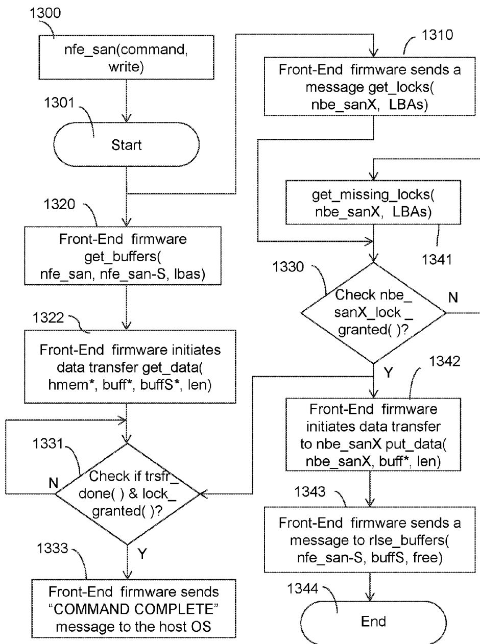
FIG. 13 nFE_SAN executes a write request write(lba, len)
