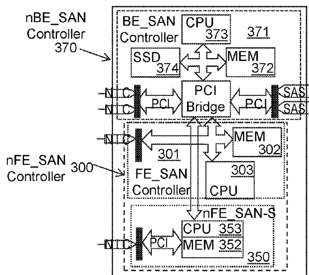
FIG. 3b nBE_SAN with integrated nFE_SAN Storage Controller
