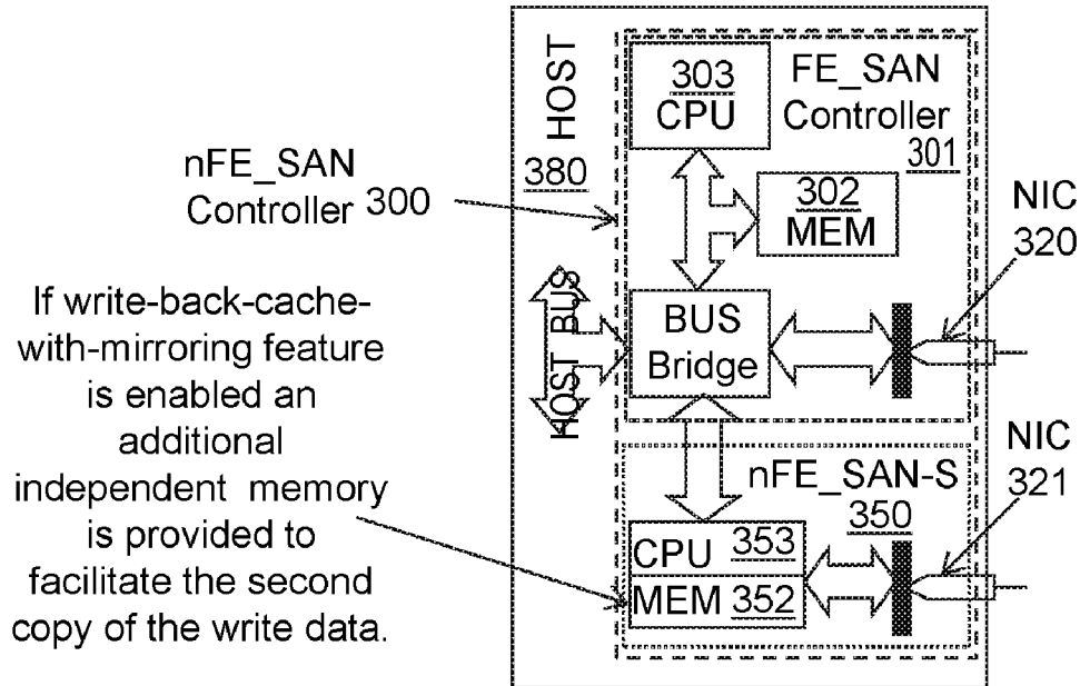
nFE_SAN Storage Controller – Write-Back -Cache with Mirroring
