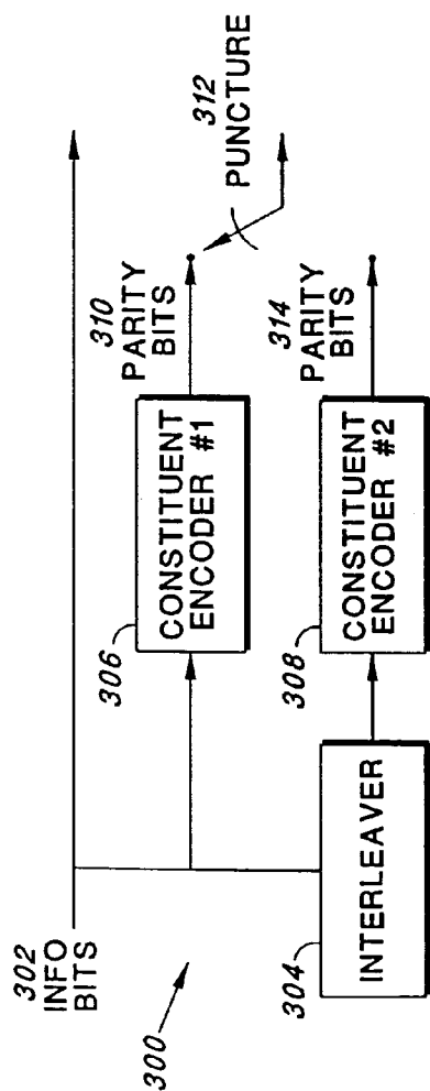
FIG. 3 GENERIC TURBO CODE ENCODER BLOCK DIAGRAM
