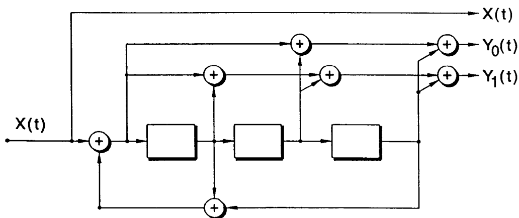
FIG. 25 CONSTITUENT ENCODER FOR REVERSE-LINK TURBO CODE
