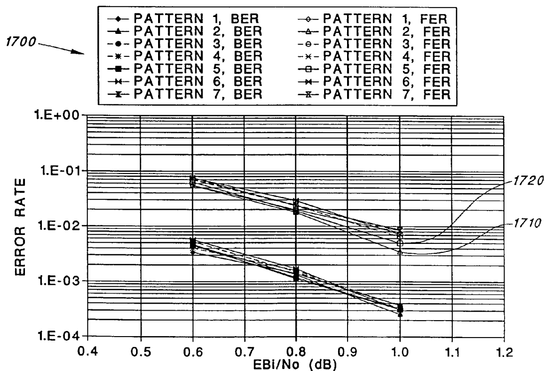
FIG. 17 COMPARISON OF RATE 1/3 PUNCTURING SCHEMES, FRAME=512
