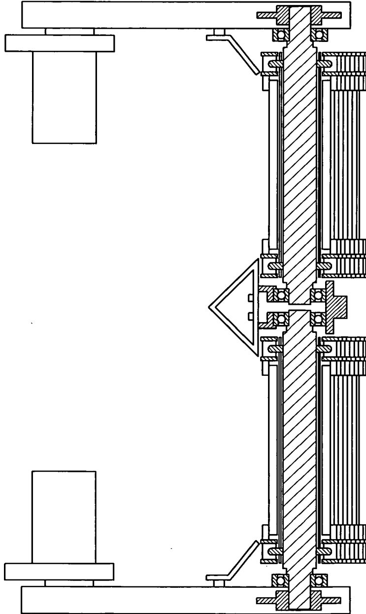
FIG. 8 (PRIOR ART)
