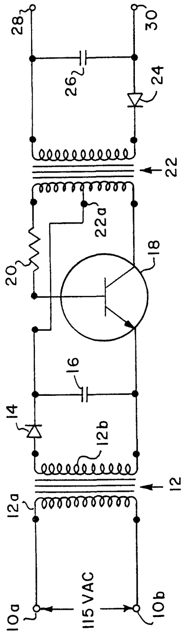
FIG. 1 (PRIOR ART)
