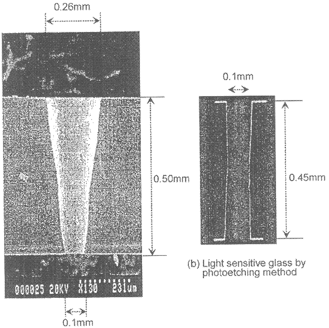
(a) Non-alkali glass by sand blasting
