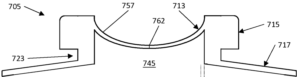
FIG. 7f SECTION C-C
