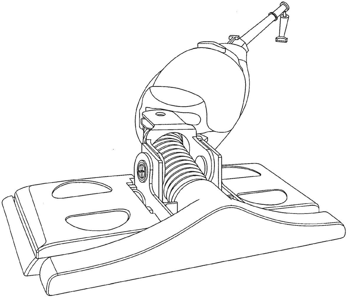
FIG. 25 (Prior Art)
