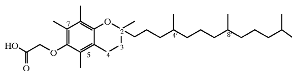
2,5,7,8-tetramethyl-(2RS,4RS,8RS, 12-trimethyltridecyl)chroman-6-yloxy)acetic acid (15)
