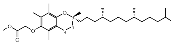
Methyl2,5,7,8-tetramethyl-(2R-(4R,8R,12-trimethyltridecyl)chroman-6-yloxy)acetate (11)
