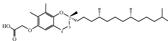
2,7,8-trimethyl-(2R-(4R,8R,12-trimethyltridecyl) chroman-6-yloxy)acetic acid (8)
