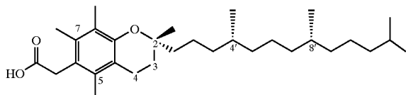
6-(2,5,7,8-tetramethyl-(2R-(4R,8,12-trimethyltridecyl)chroman)acetic acid (22)
