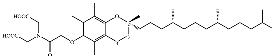
2-(N,N-(carboxymethyl)-2(2,5,7,8-tetramethyl-(2R-(4R,8R,12-trimethyltridecyl)chroman-6-yloxy)acetic acid (12)
