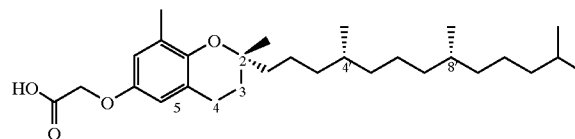
2,8-dimethyl-(2R-(4R,8R,12-trimethyltridecyl) chroman-6-yloxy)acetic acid (9)
