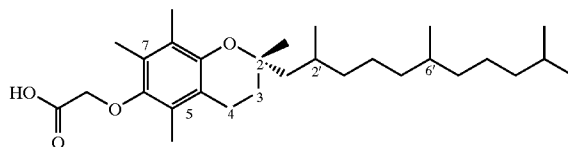
2,5,7,8-tetramethyl-2R-(2RS,6RS, 10-trimethylundecyl)chroman-6-yloxy)acetic acid (17)
