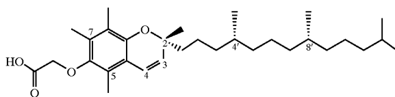
2,5,7,8-tetramethyl-(2R-(4R,8R,12-trimethyltridecyl)chroman-3-ene-6-yloxy) acetic acid (20)
