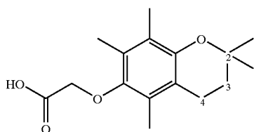
2-(2,5,7,8-pentamethylchroman-6-yloxy)acetic acid (14)
