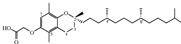
2,5,8-trimethyl-(2R-(4R,8R,12-trimethyltridecyl) chroman-6-yloxy)acetic acid (7)
