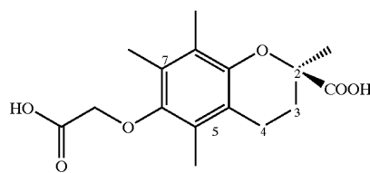
2,5,7,8-tetramethyl-(2R-(carboxy)chroman-6-yloxy)) acetic acid (16)
