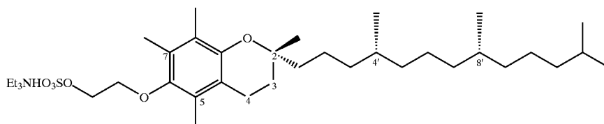
2-(2,5,7,8-tetramethyl-(2R-(4R,8R,12-trimethyltridecyl)chroman-6-yloxy) triethylammonium sulfate (21)
