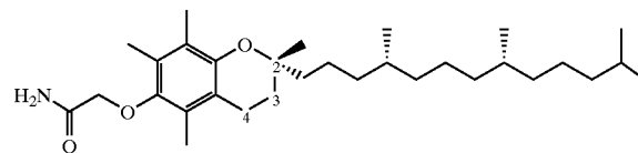
2,5,7,8-tetramethyl-(2R-(4R,8R,12-trimethyltridecyl)chroman-6-yloxy)acetamide (10)
