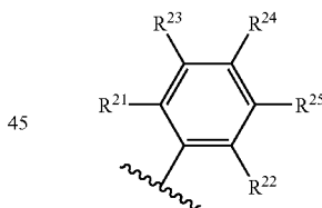
Formula (IVa)
