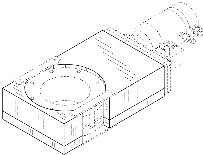
立體圖1
