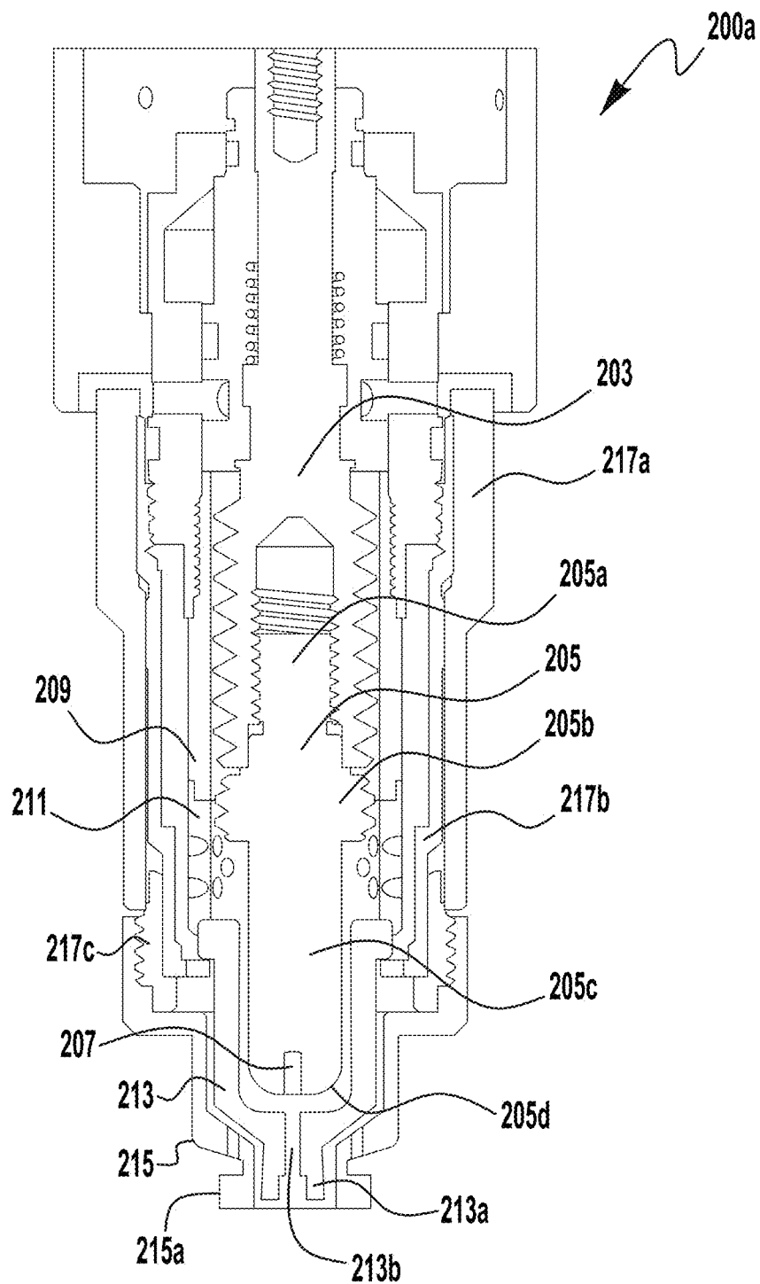
FIG. 2 PRIOR ART
