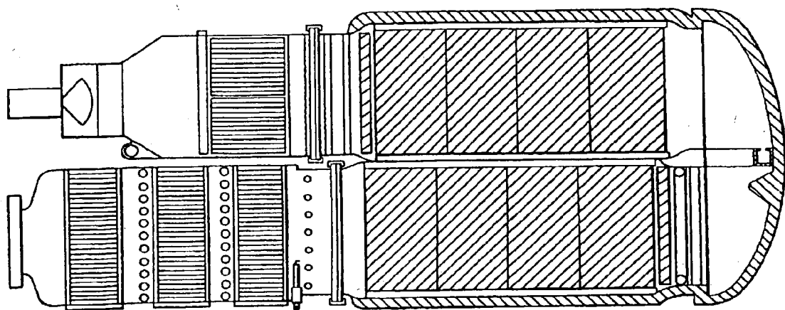
FIG. 6 PRIOR ART
