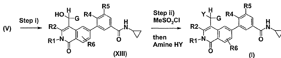
Scheme 6
