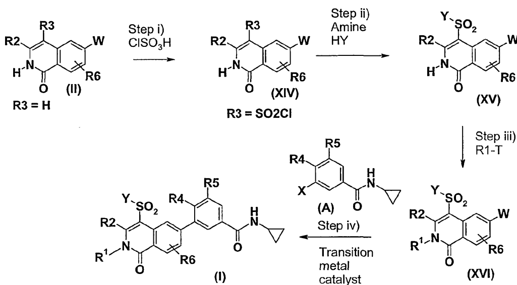
10 Scheme 7
