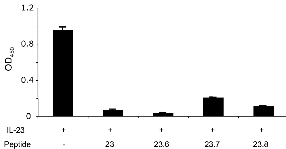
Competitive ELISA
