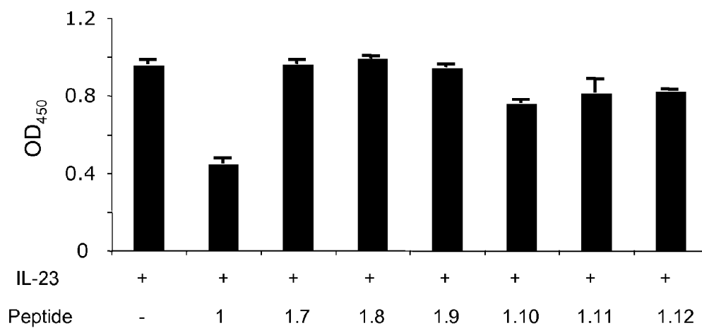
Competitive ELISA
