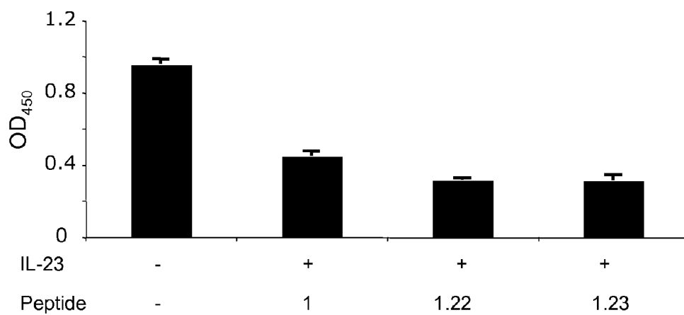
Competitive ELISA
