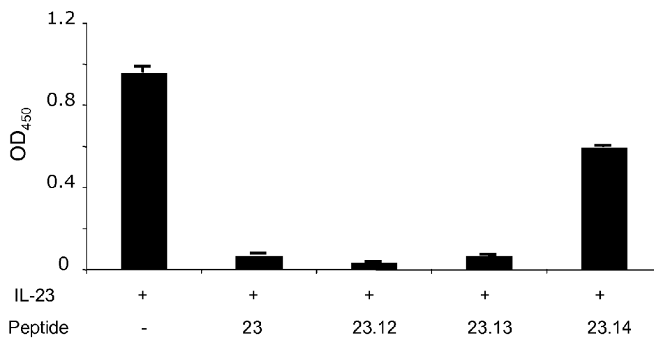
Competitive ELISA
