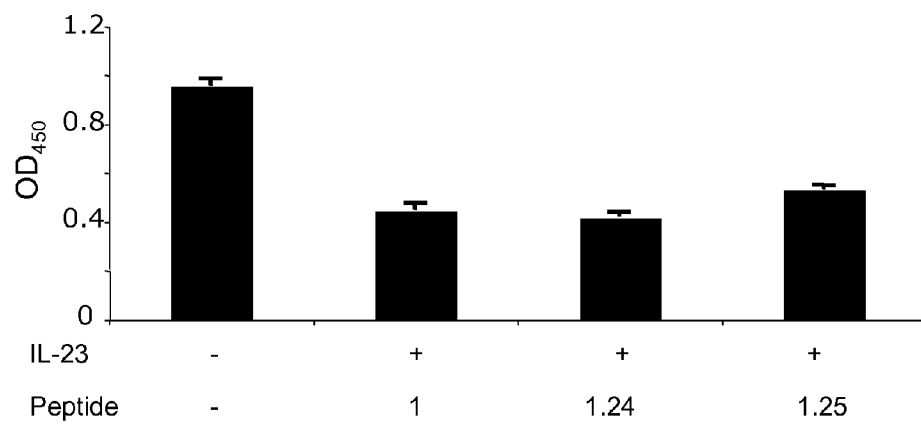
Competitive ELISA
