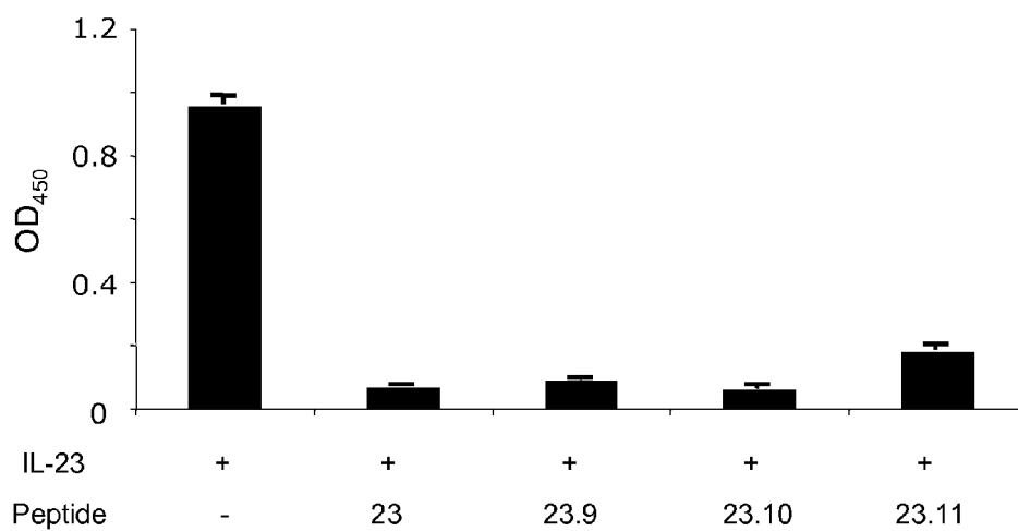
Competitive ELISA
