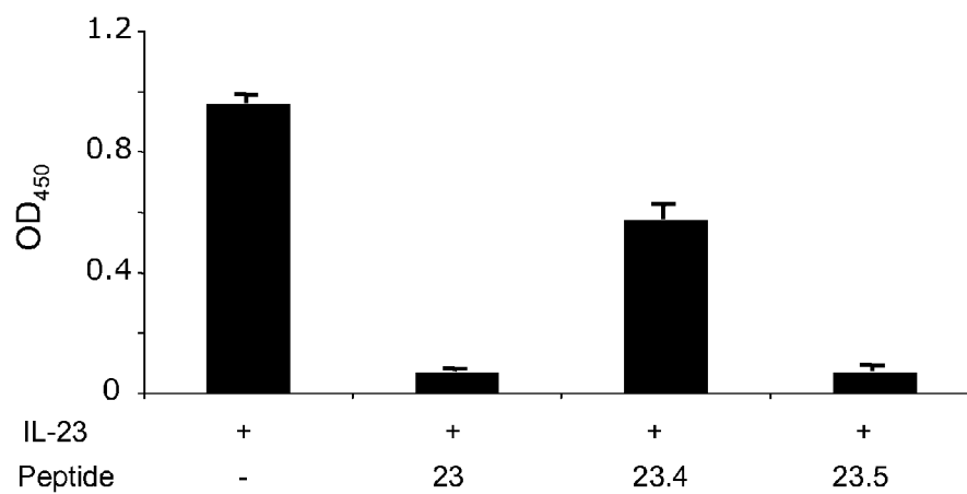
Competitive ELISA
