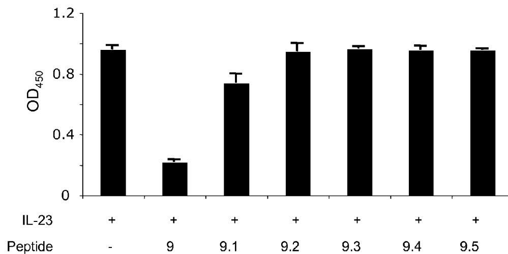
Competitive ELISA
