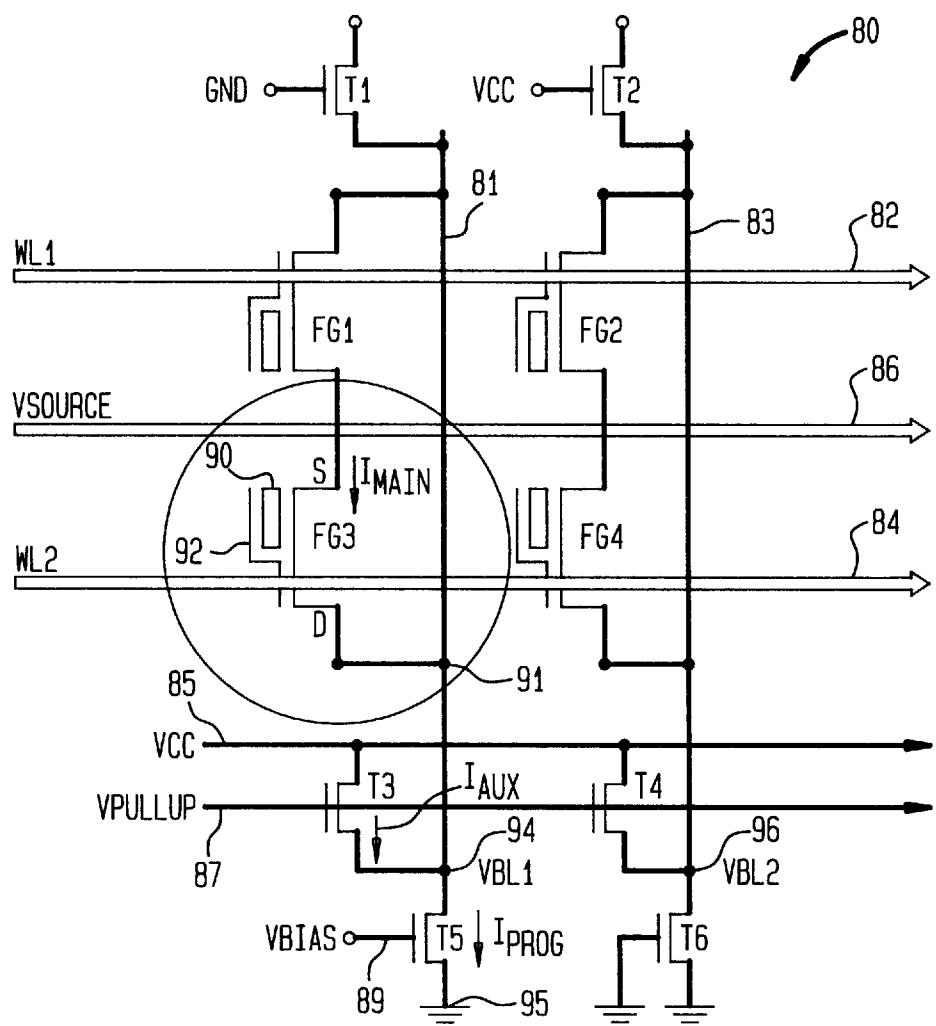
FIG. 8 (PRIOR ART)
