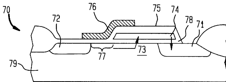
FIG. 7 (PRIOR ART)
