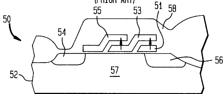
FIG. 5 (PRIOR ART)
