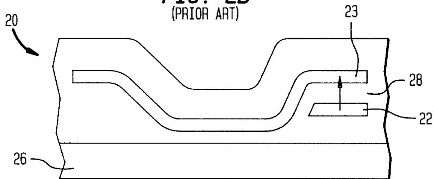
FIG. 3 (PRIOR ART)
