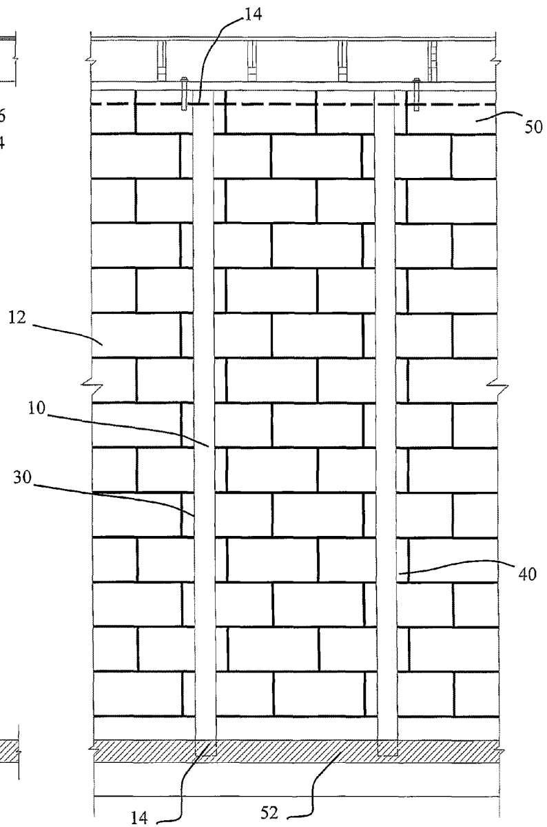
Elevation of inside face of wall
