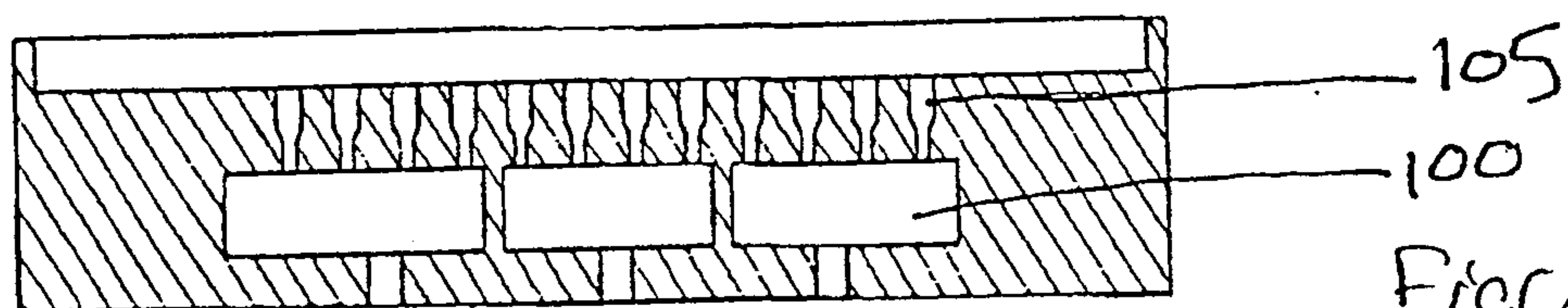
Fig. 2 Base Block Concept, Cross Section Side View
