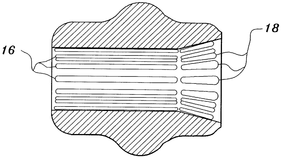
( VIEW 2-2 )
