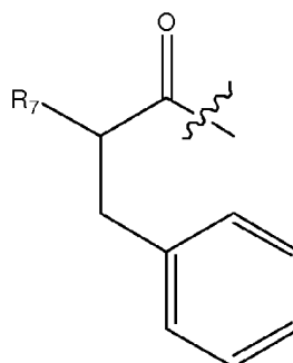
Formula XI
