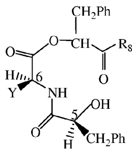
3: L,L-dipeptide extension
