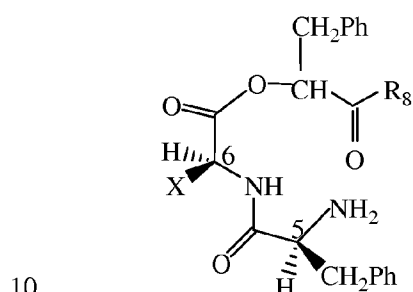
1: L,L-dipeptide extension
