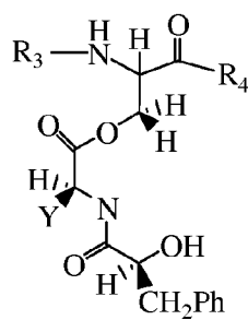
4: L,L-dipeptide extension
