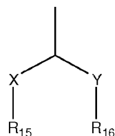
Formula VII
