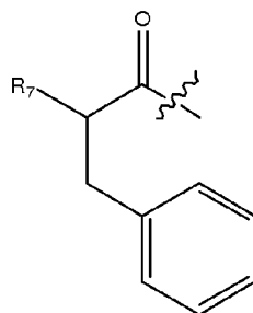
Formula XI
