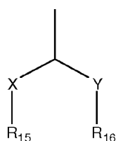
Formula VII
