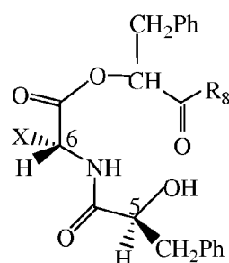
2: L,D-dipeptide extension
