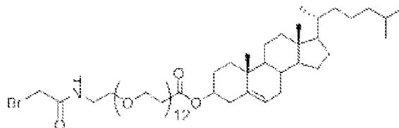
Br-Oxa 12 -Chole
