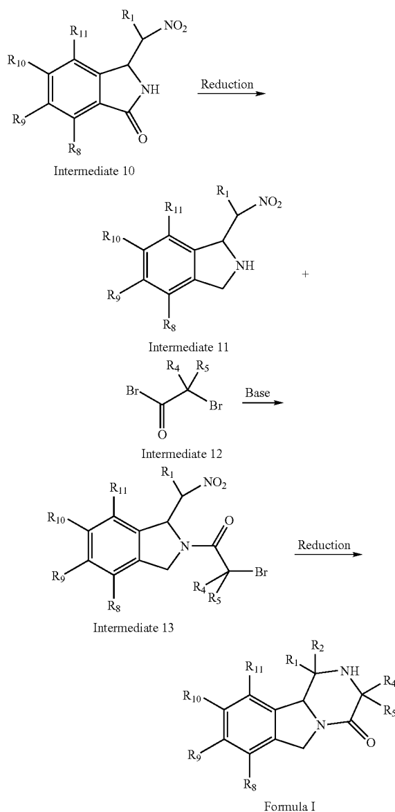
SCHEME 3
