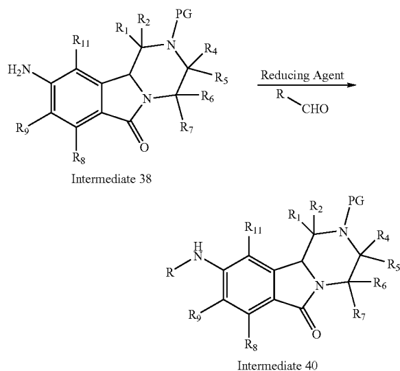
SCHEME 15
