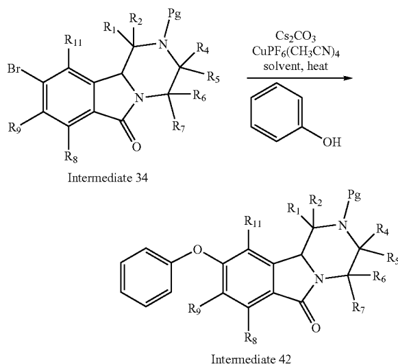
SCHEME 17
