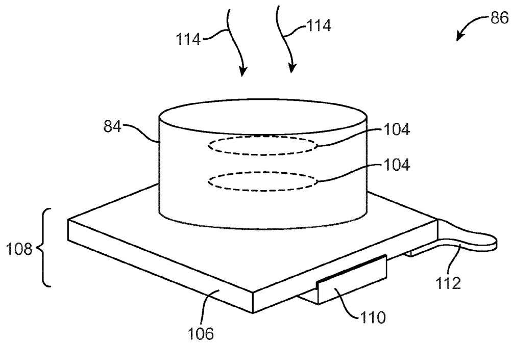
(PRIOR ART) FIG. 7
