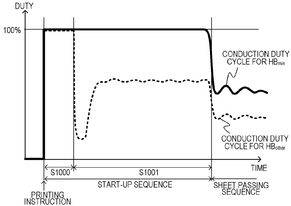
FIG. 6B CONDUCTION DUTY CYCLE
