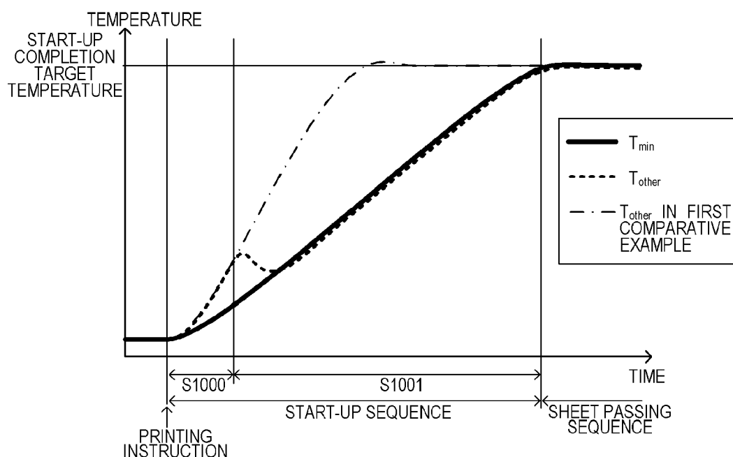
FIG. 6A THERMISTOR TH DETECTION TEMPERATURE
