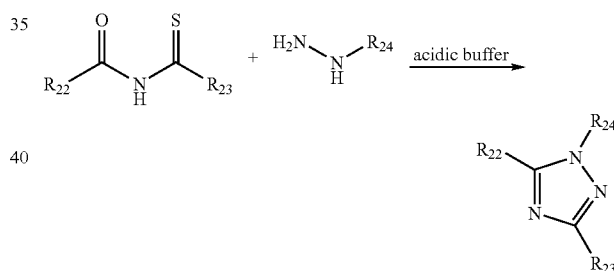
Scheme V: Formation of a triazole.
