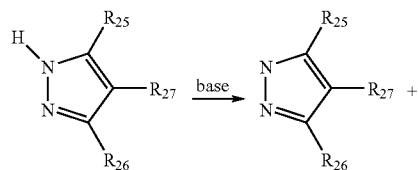
Scheme IV: Formation of a substitute 1-(pyridin-2-yl)pyrazole.
