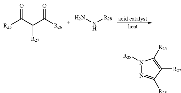
Scheme I: Formation of pyrazole ring.
