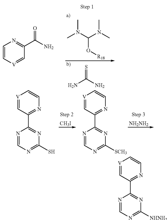
Scheme III: Formation of a substituted 2-hydrazinotriazine
