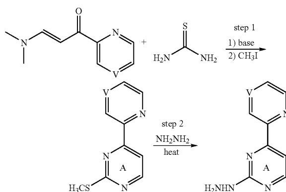
Scheme II: Preparation of substituted 2-hydrazinopyrimidine.
