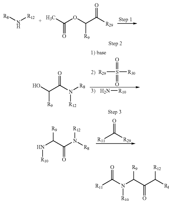
Scheme VII: Formation of compounds represented by Formula III.
