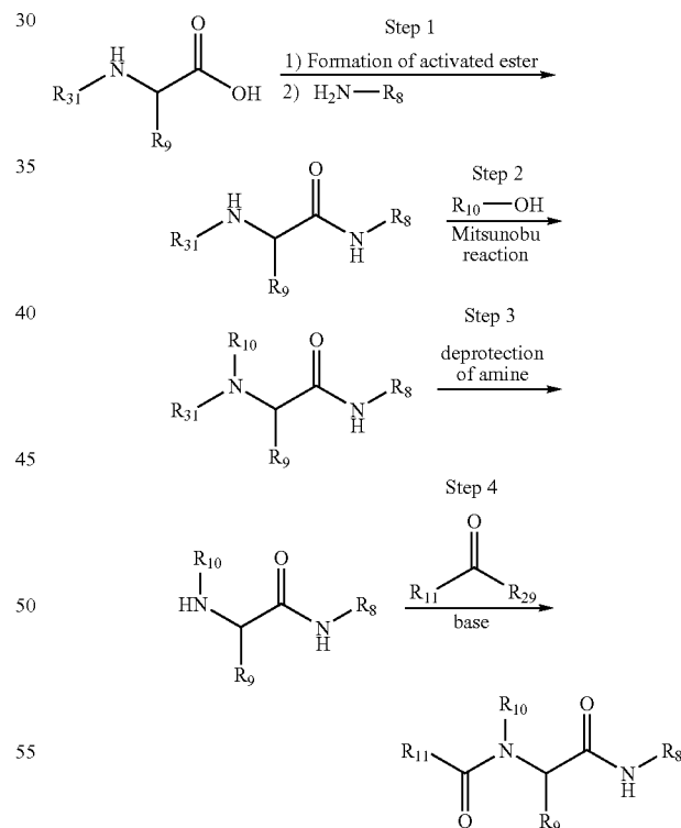
Scheme VIII: Third method of forming the compounds represented by Formula III.
