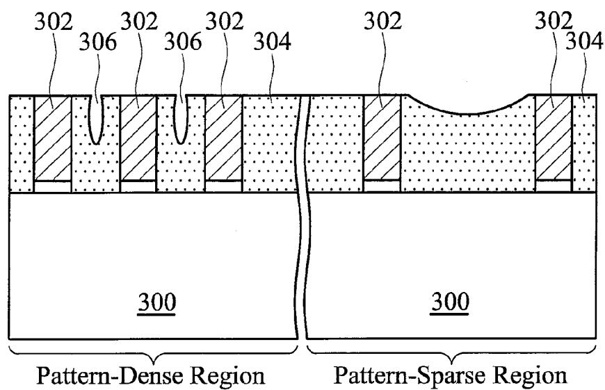
FIG. 3 (PRIOR ART)
