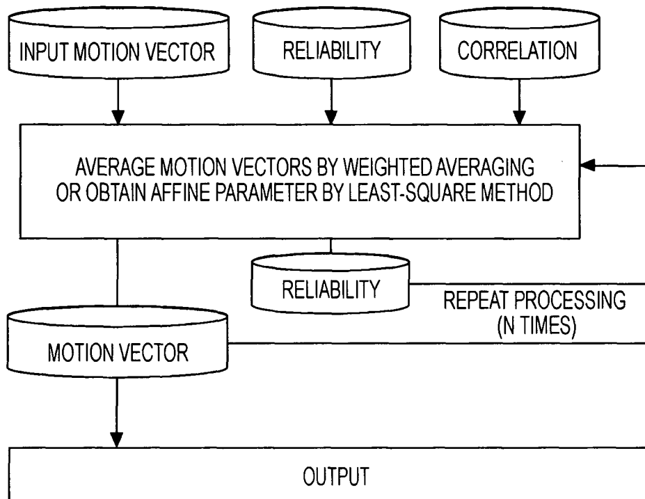
FLOWCHART OF SMOOTHING PROCESSING
