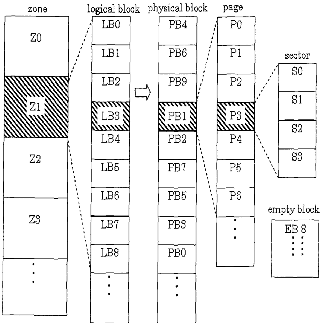
Fig.2 (Prior Art)
