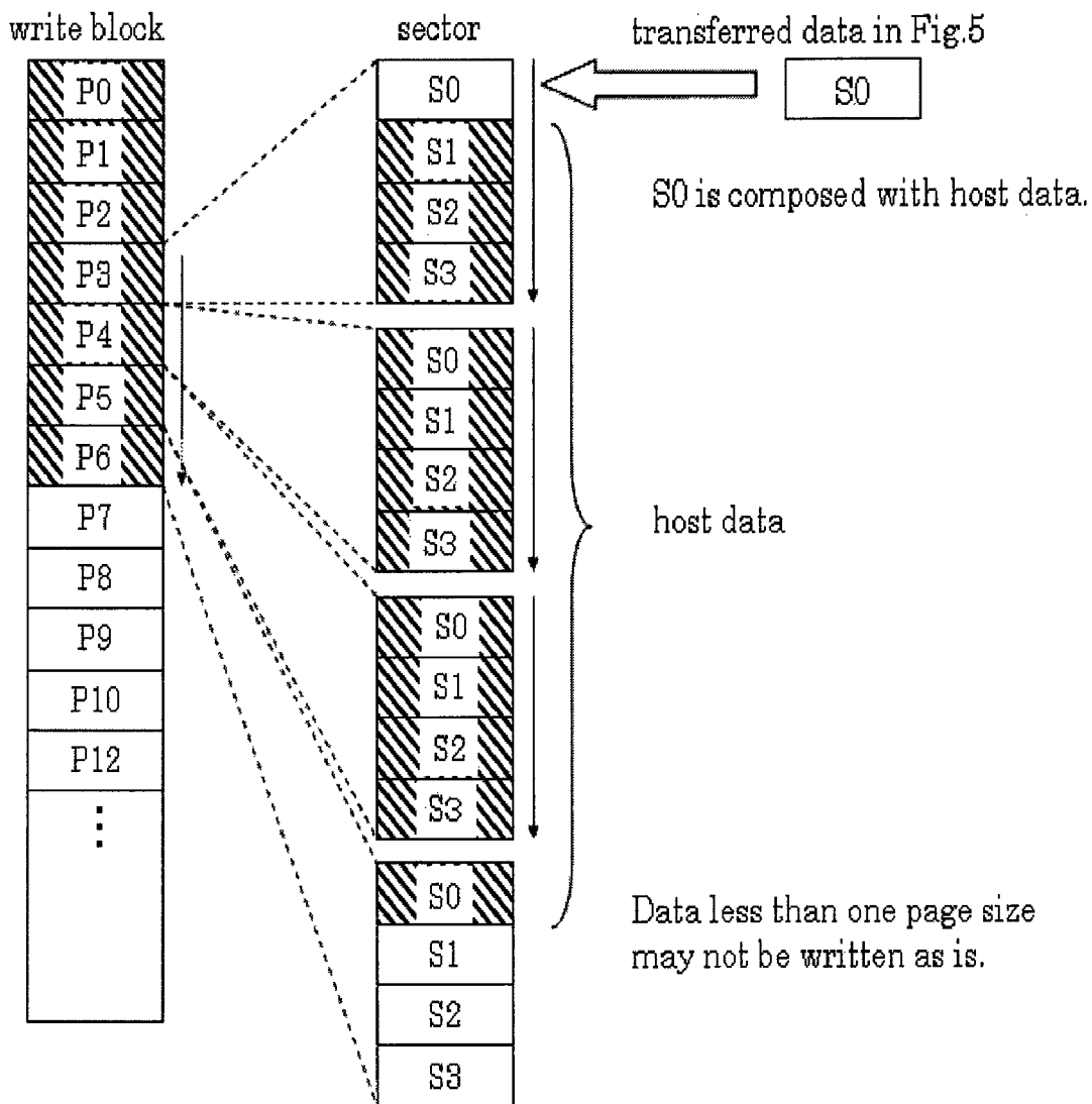
Fig.6 (Prior Art)
