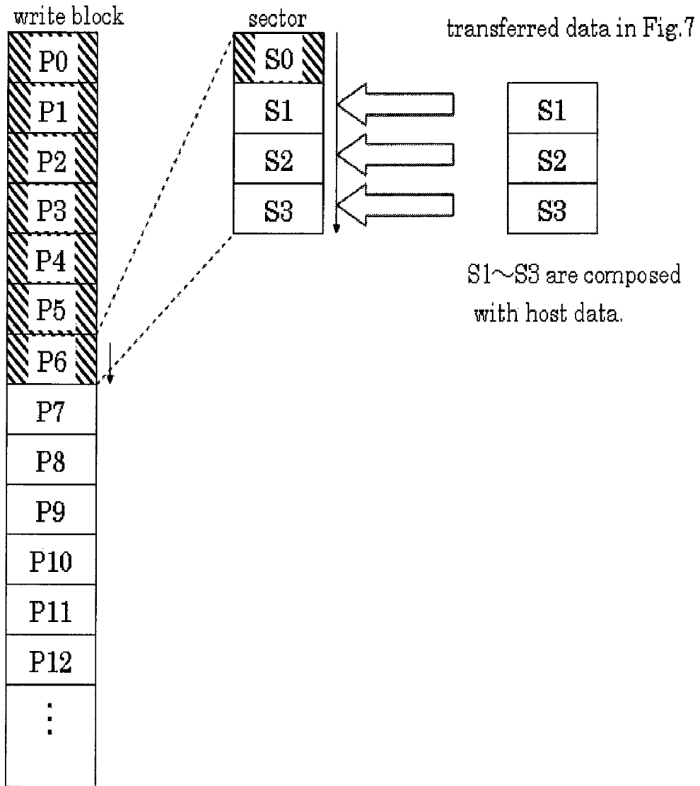
Fig.8 (Prior Art)
