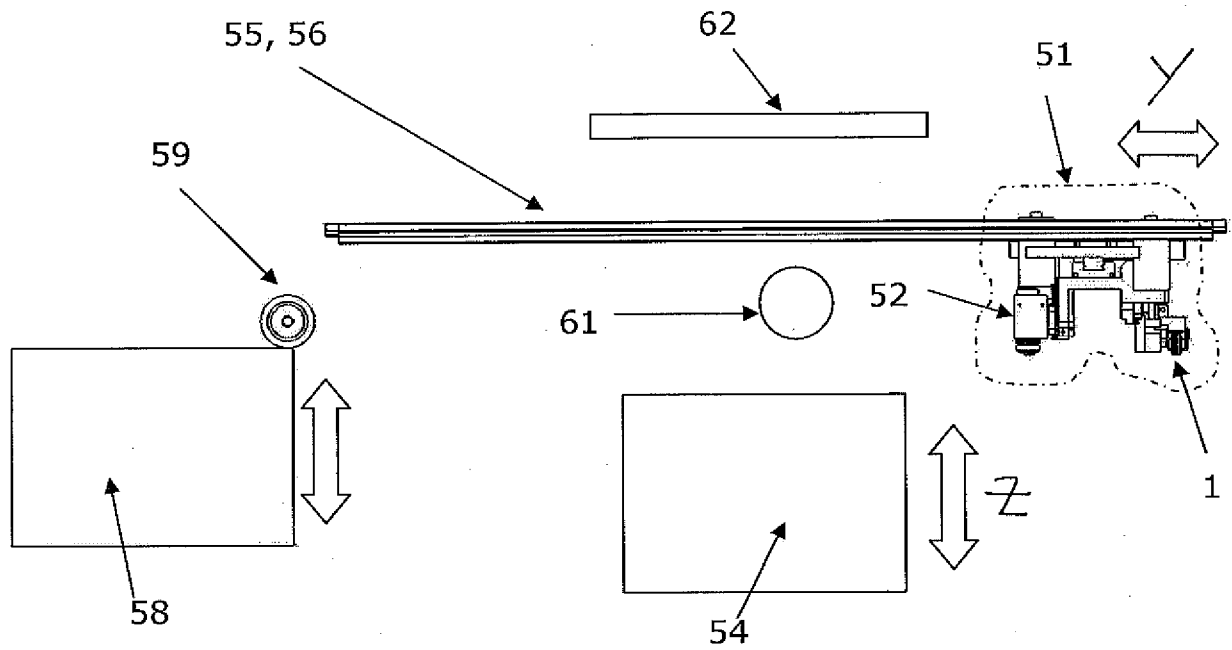
Figure 7: Basic Machine Layout: Front Elevation
