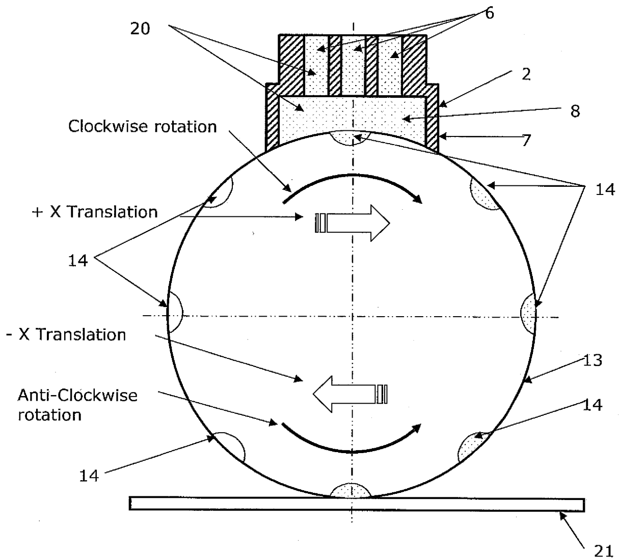
Figure 5: Priming of the adhesive wheel
