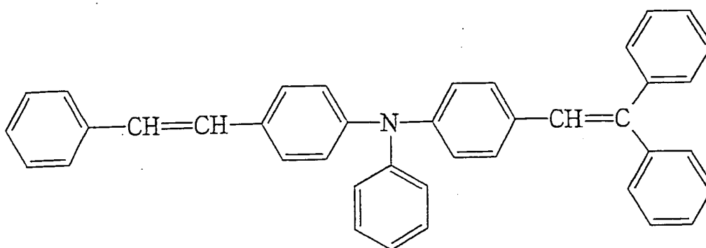
Structural Formula (2)
