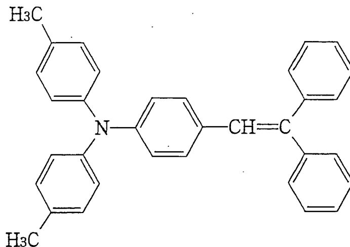
Structural Formula (1)
