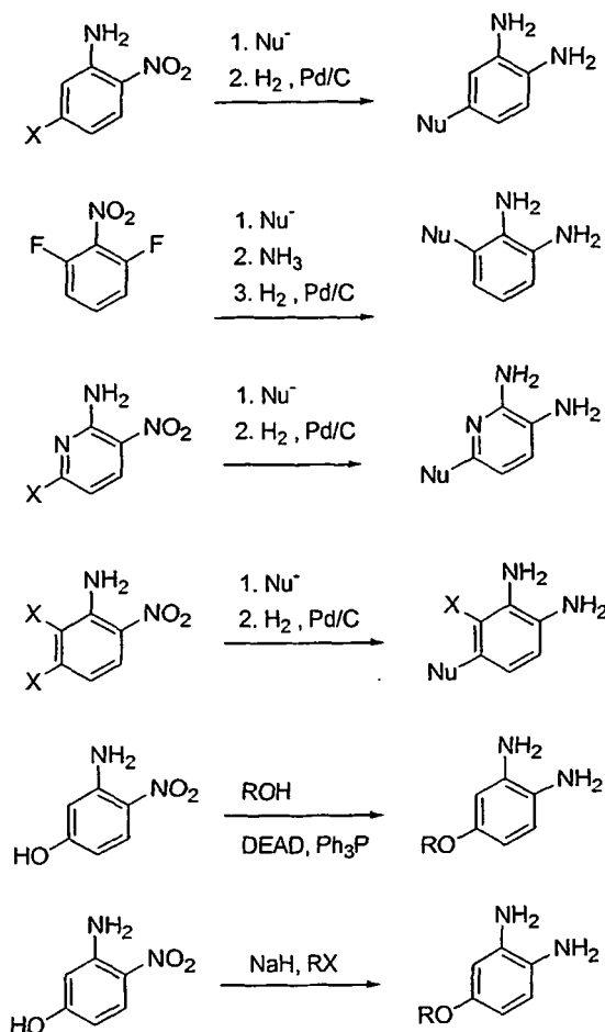
Scheme 5.
