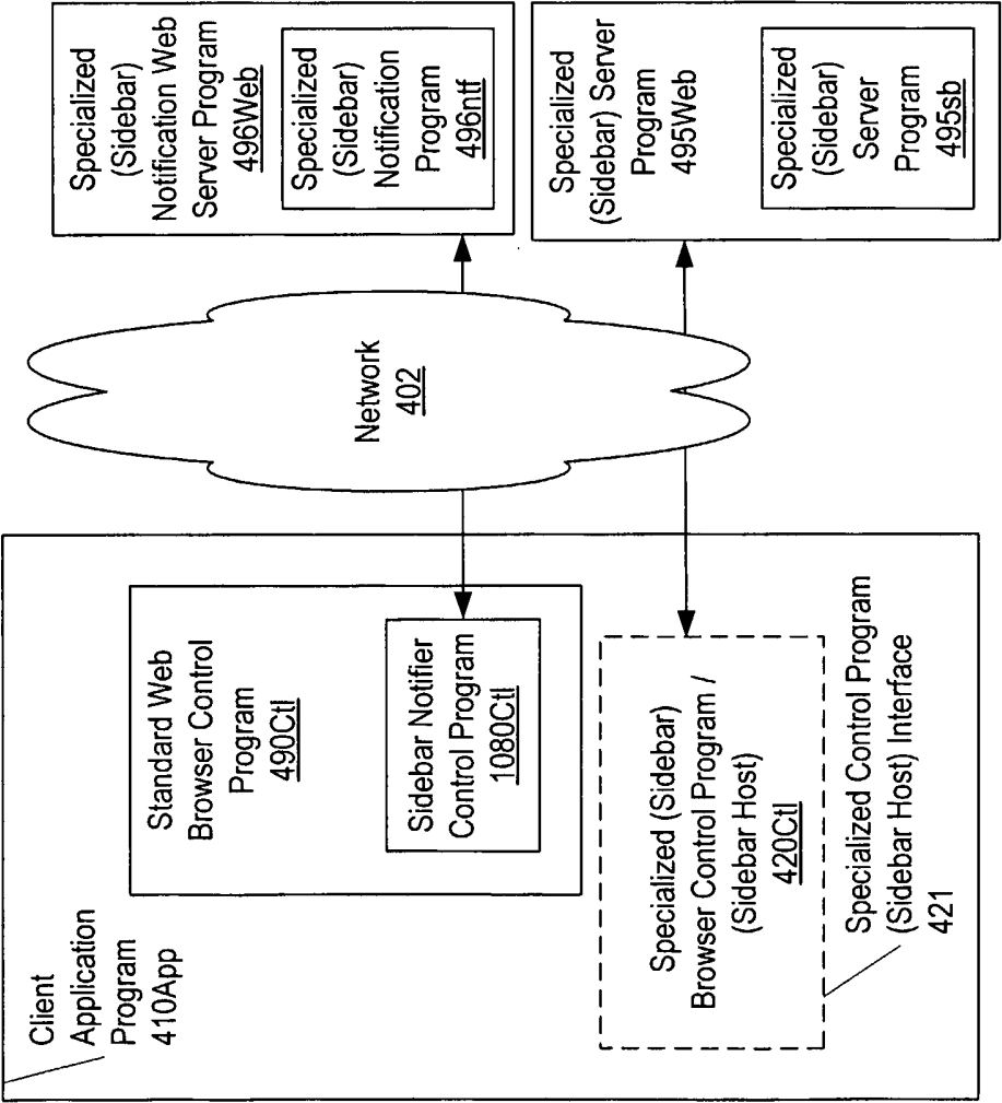
Alternative Software Architecture Fig. 10A
