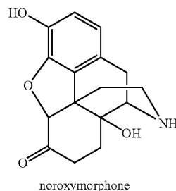
noroxymorphone
