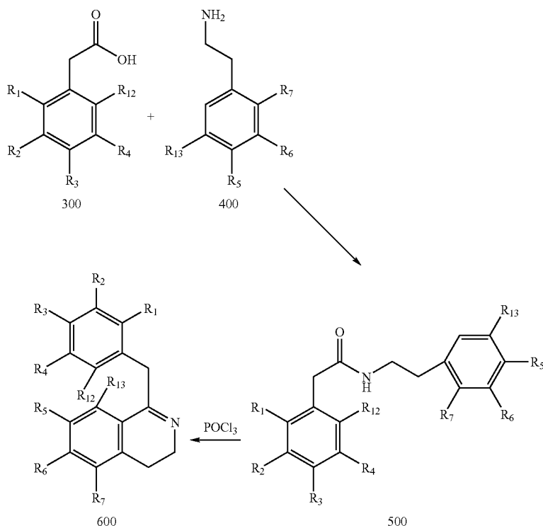
Reaction Scheme 1
