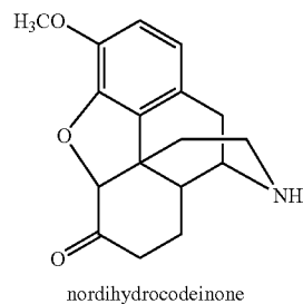
nordihydrocodeinone
