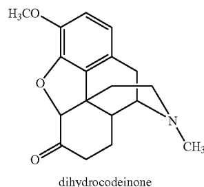
dihydrocodeinone
