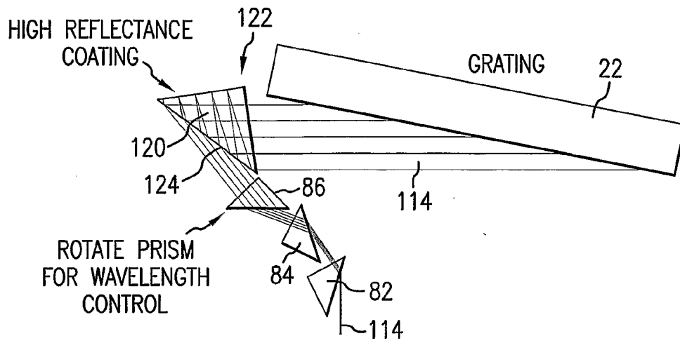
OPTICAL DESIGN FOR COMPACT LNM ROBERT BERGSTEDT 5/27/04
