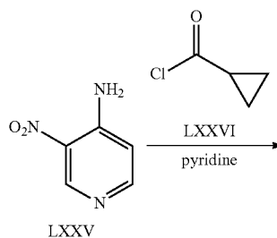
Scheme 13
