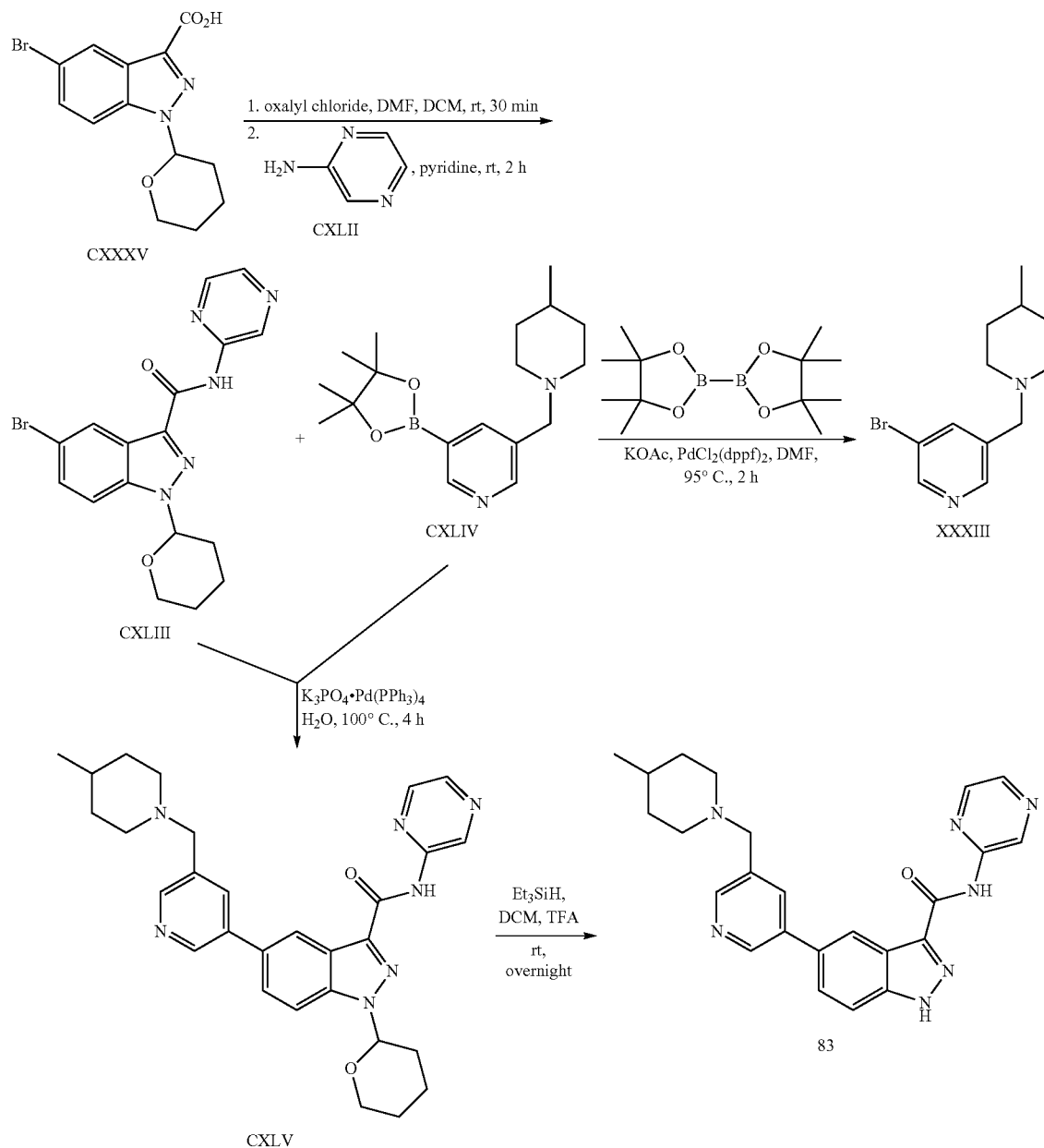
Scheme 27
