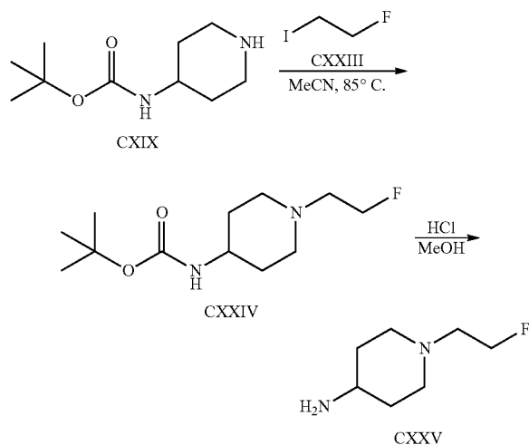
Scheme 24
