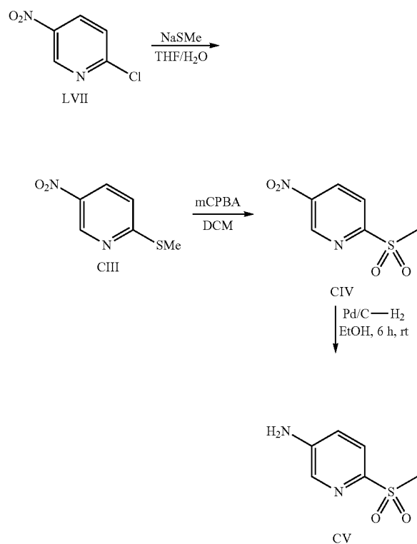
Scheme 19
