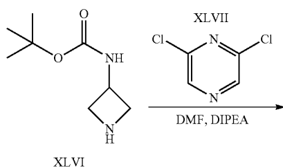
Scheme 7
