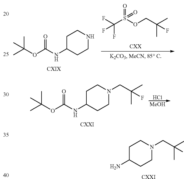
Scheme 23
