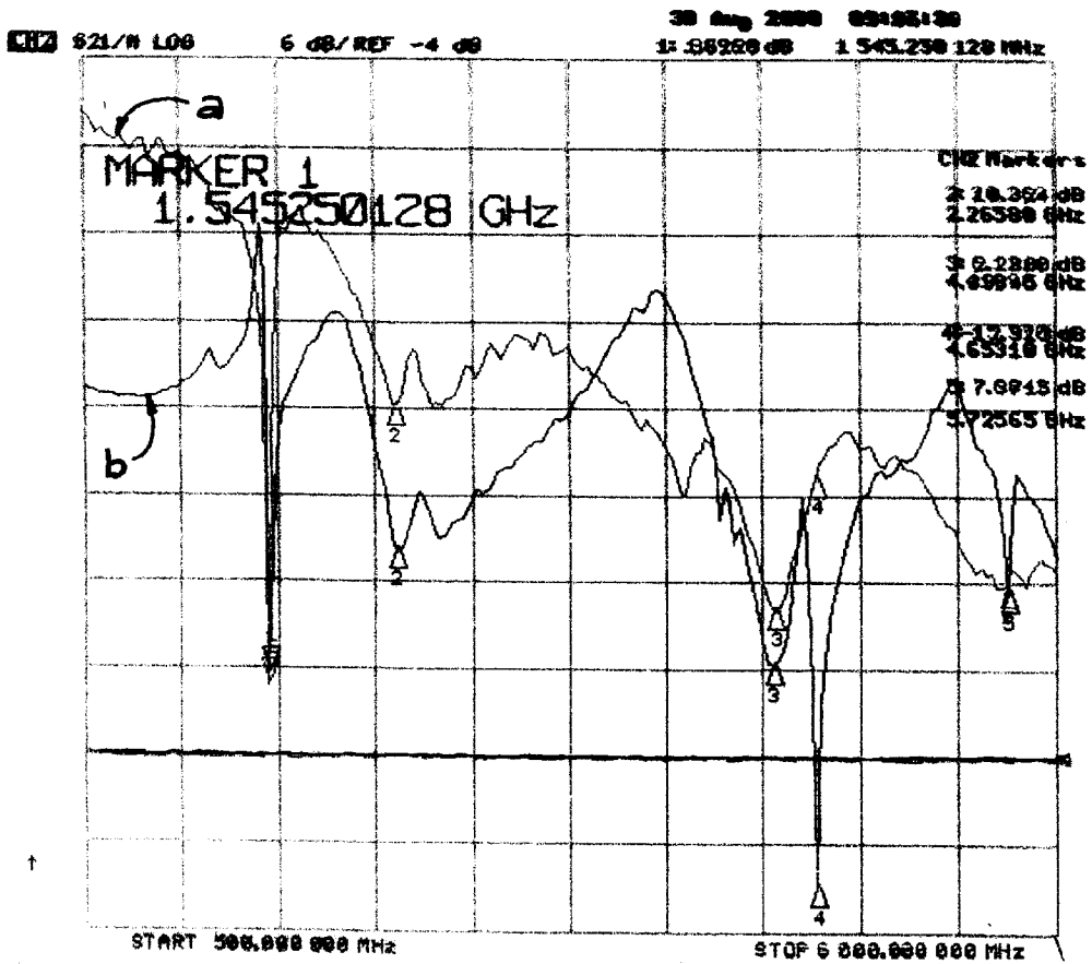
(a) RE-ENTRANT CAVITY TRANSMISSION RESPONSE (b) COAXIAL CAVITY TRANSMISSION RESPONSE FIG. 3
