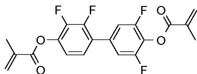
RM-5
