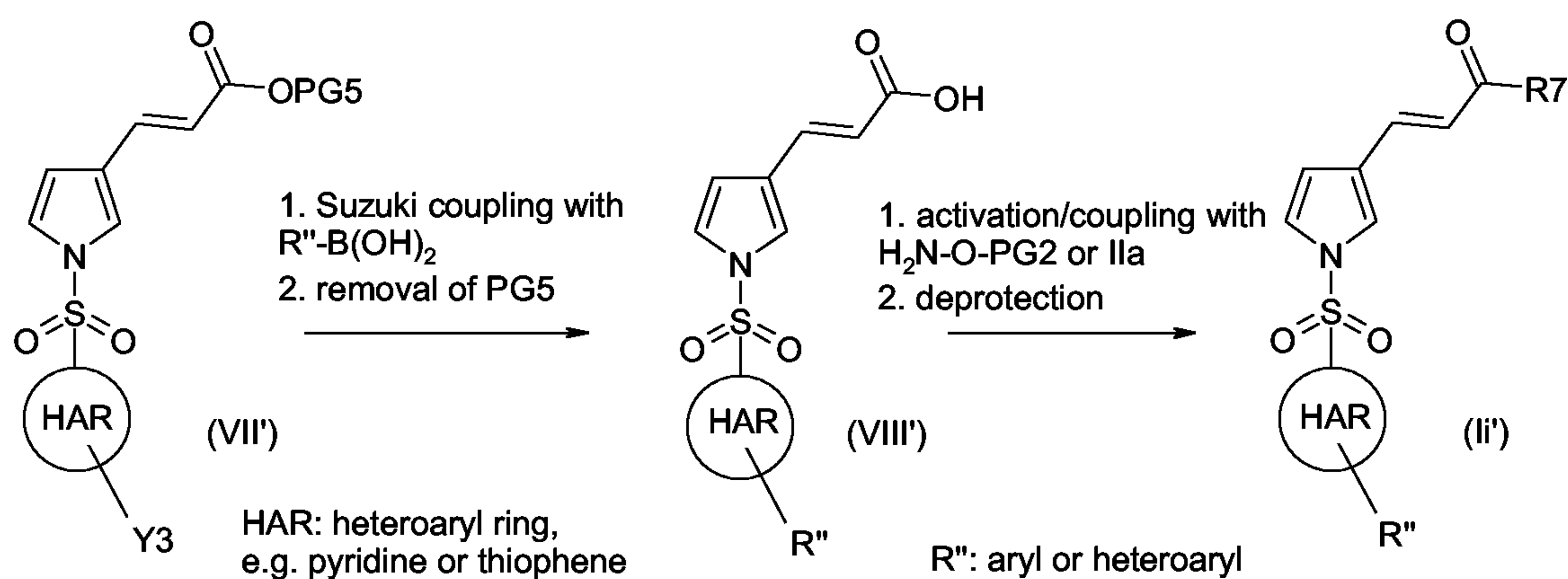
Reaction scheme 5:
