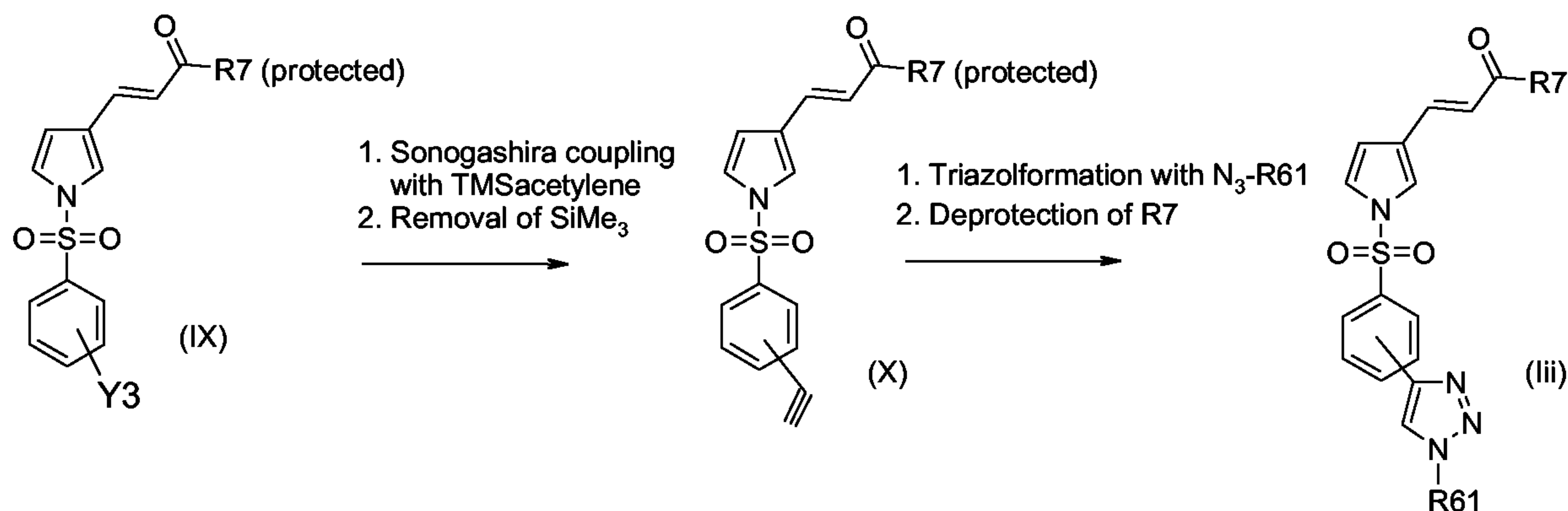
Reaction scheme 6:
